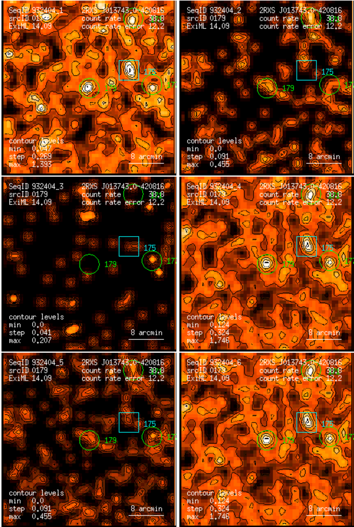
Figure 179: RASS 932404: detection 0179: band rate images, Gaussian filter: (1) PSPC channels 11 – 41, (2) 52 – 90, (3) 91 – 201, (4) 11 – 235, (5) 52 – 201, (6) 11 – 201. Broad band rates in counts/ks. Band rate contour levels in counts/ks/arcmin 2 .
