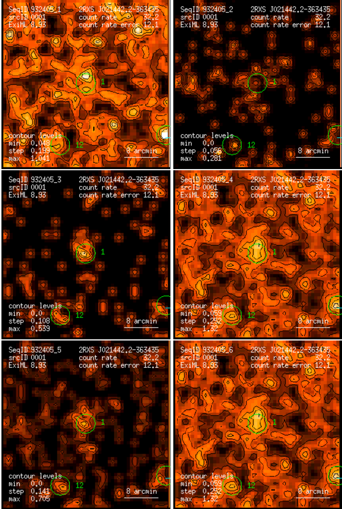
Figure 1: RASS 932405: detection 0001: band rate images, Gaussian filter: (1) PSPC channels 11 – 41, (2) 52 – 90, (3) 91 – 201, (4) 11 – 235, (5) 52 – 201, (6) 11 – 201. Broad band rates in counts/ks. Band rate contour levels in counts/ks/arcmin 2 .
