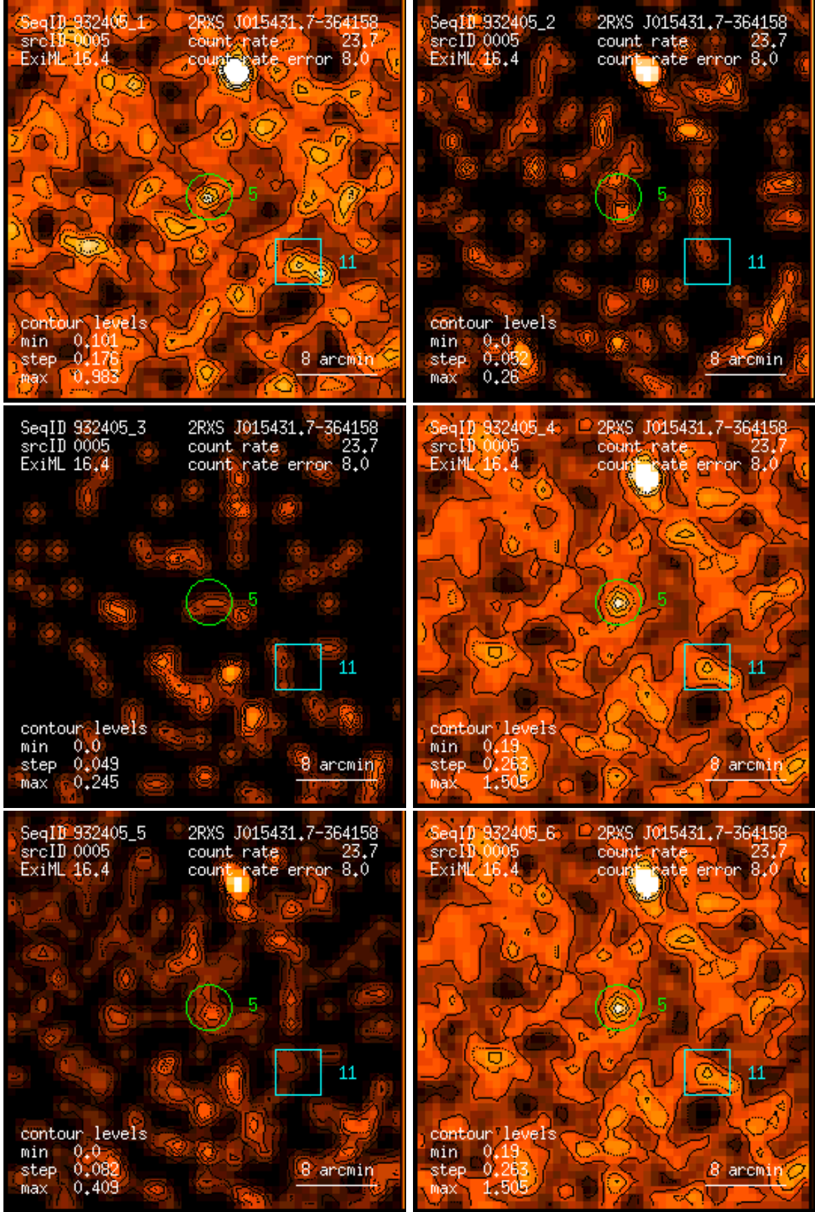
Figure 5: RASS 932405: detection 0005: band rate images, Gaussian filter: (1) PSPC channels 11 – 41, (2) 52 – 90, (3) 91 – 201, (4) 11 – 235, (5) 52 – 201, (6) 11 – 201. Broad band rates in counts/ks. Band rate contour levels in counts/ks/arcmin 2 .
