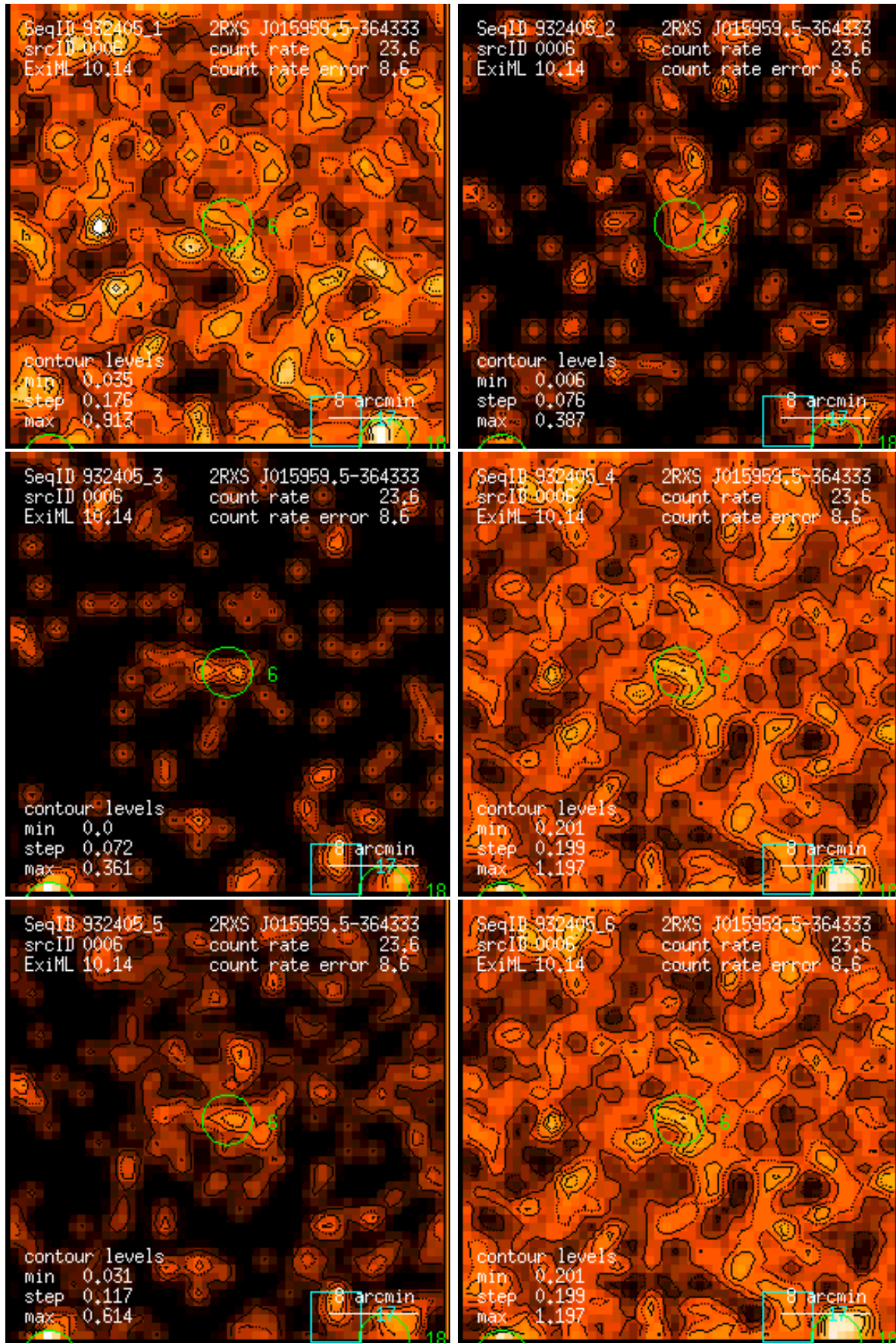
Figure 6: RASS 932405: detection 0006: band rate images, Gaussian filter: (1) PSPC channels 11 – 41, (2) 52 – 90, (3) 91 – 201, (4) 11 – 235, (5) 52 – 201, (6) 11 – 201. Broad band rates in counts/ks. Band rate contour levels in counts/ks/arcmin 2 .
