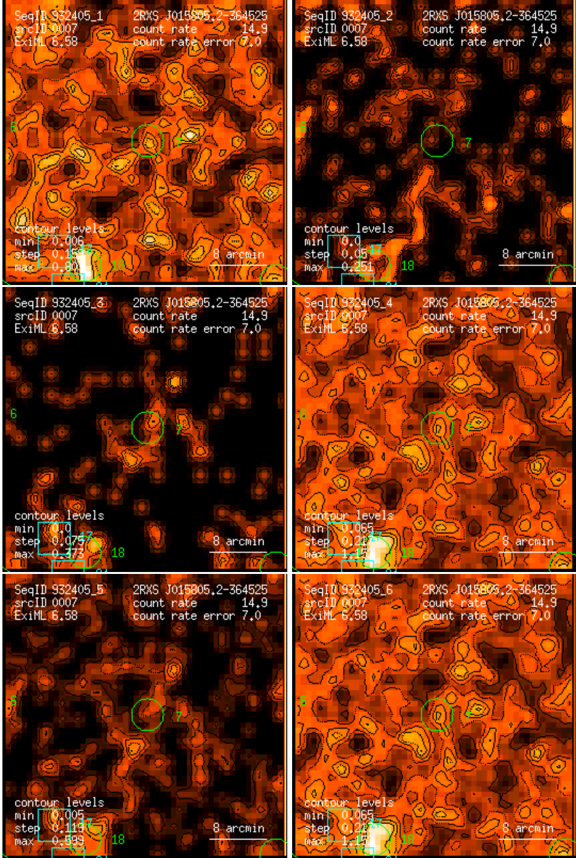
Figure 7: RASS 932405: detection 0007: band rate images, Gaussian filter: (1) PSPC channels 11 – 41, (2) 52 – 90, (3) 91 – 201, (4) 11 – 235, (5) 52 – 201, (6) 11 – 201. Broad band rates in counts/ks. Band rate contour levels in counts/ks/arcmin 2 .
