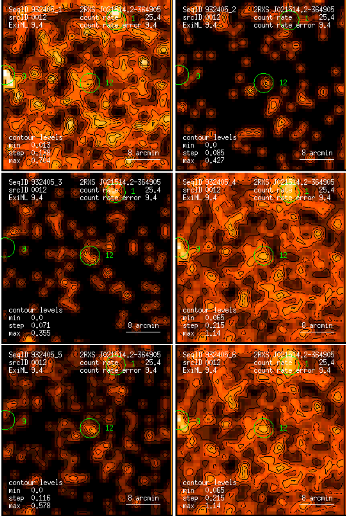
Figure 12: RASS 932405: detection 0012: band rate images, Gaussian filter: (1) PSPC channels 11 – 41, (2) 52 – 90, (3) 91 – 201, (4) 11 – 235, (5) 52 – 201, (6) 11 – 201. Broad band rates in counts/ks. Band rate contour levels in counts/ks/arcmin 2 .
