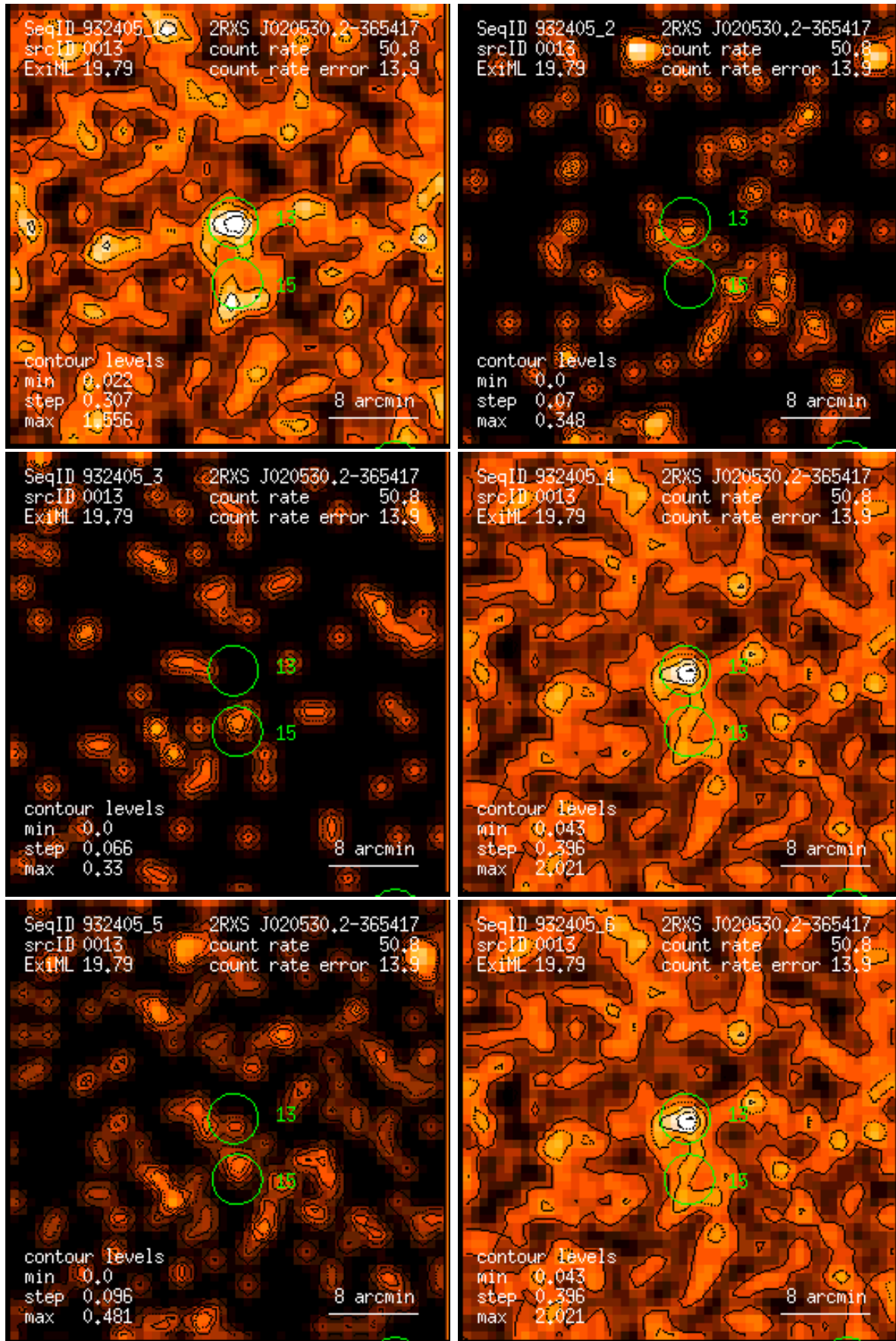
Figure 13: RASS 932405: detection 0013: band rate images, Gaussian filter: (1) PSPC channels 11 – 41, (2) 52 – 90, (3) 91 – 201, (4) 11 – 235, (5) 52 – 201, (6) 11 – 201. Broad band rates in counts/ks. Band rate contour levels in counts/ks/arcmin 2 .
