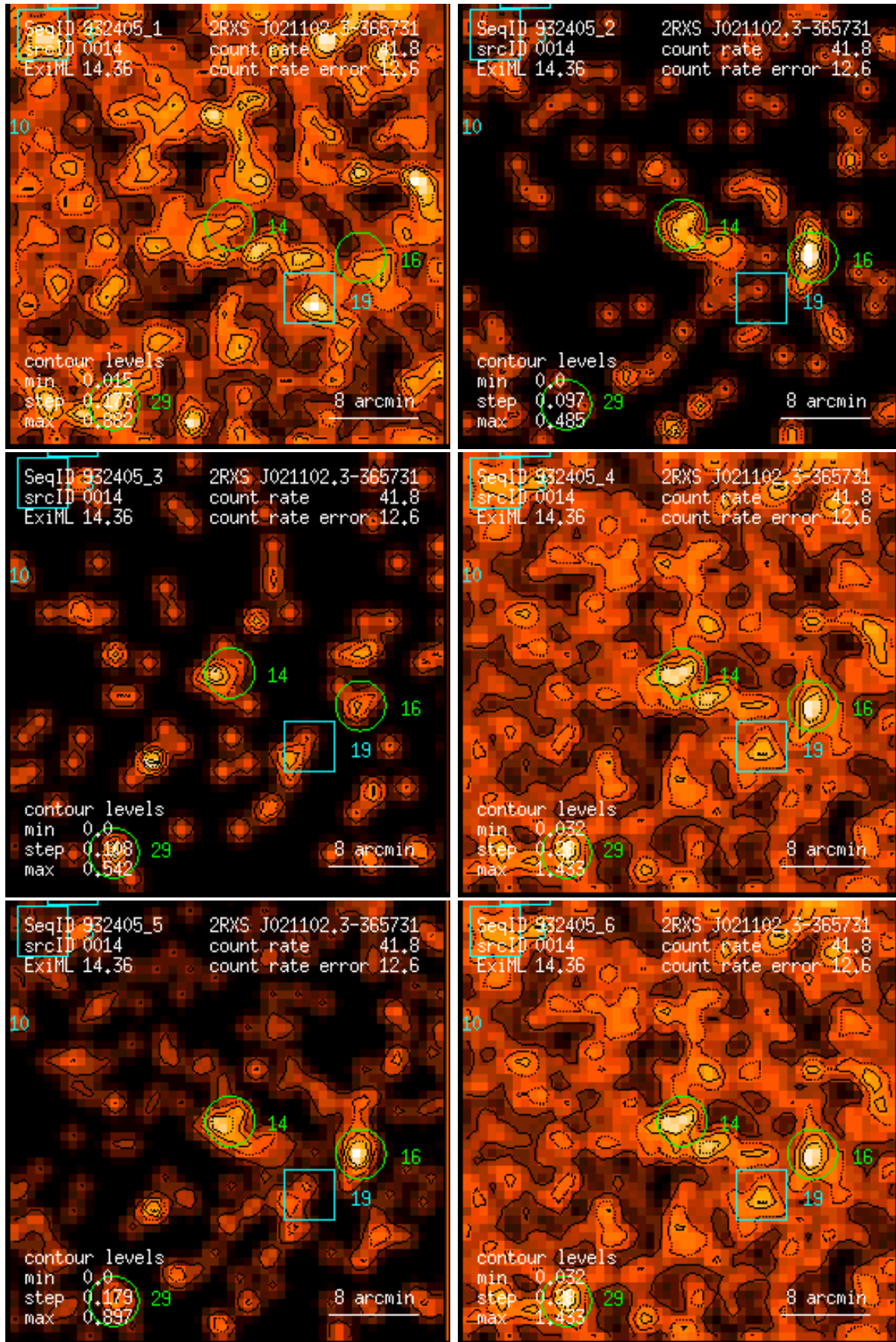
Figure 14: RASS 932405: detection 0014: band rate images, Gaussian filter: (1) PSPC channels 11 – 41, (2) 52 – 90, (3) 91 – 201, (4) 11 – 235, (5) 52 – 201, (6) 11 – 201. Broad band rates in counts/ks. Band rate contour levels in counts/ks/arcmin 2 .
