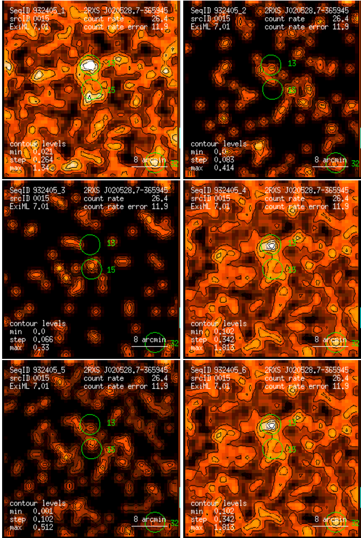
Figure 15: RASS 932405: detection 0015: band rate images, Gaussian filter: (1) PSPC channels 11 – 41, (2) 52 – 90, (3) 91 – 201, (4) 11 – 235, (5) 52 – 201, (6) 11 – 201. Broad band rates in counts/ks. Band rate contour levels in counts/ks/arcmin 2 .
