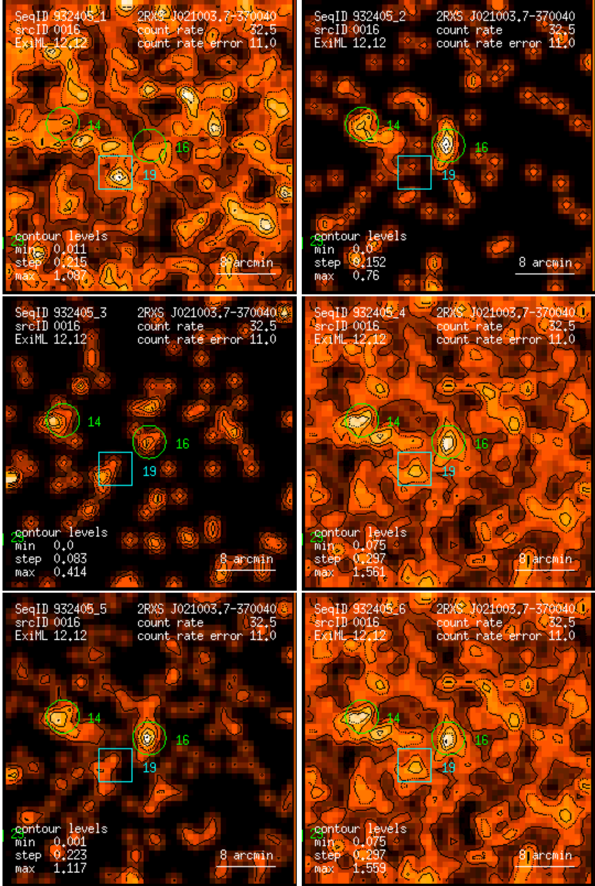
Figure 16: RASS 932405: detection 0016: band rate images, Gaussian filter: (1) PSPC channels 11 – 41, (2) 52 – 90, (3) 91 – 201, (4) 11 – 235, (5) 52 – 201, (6) 11 – 201. Broad band rates in counts/ks. Band rate contour levels in counts/ks/arcmin 2 .
