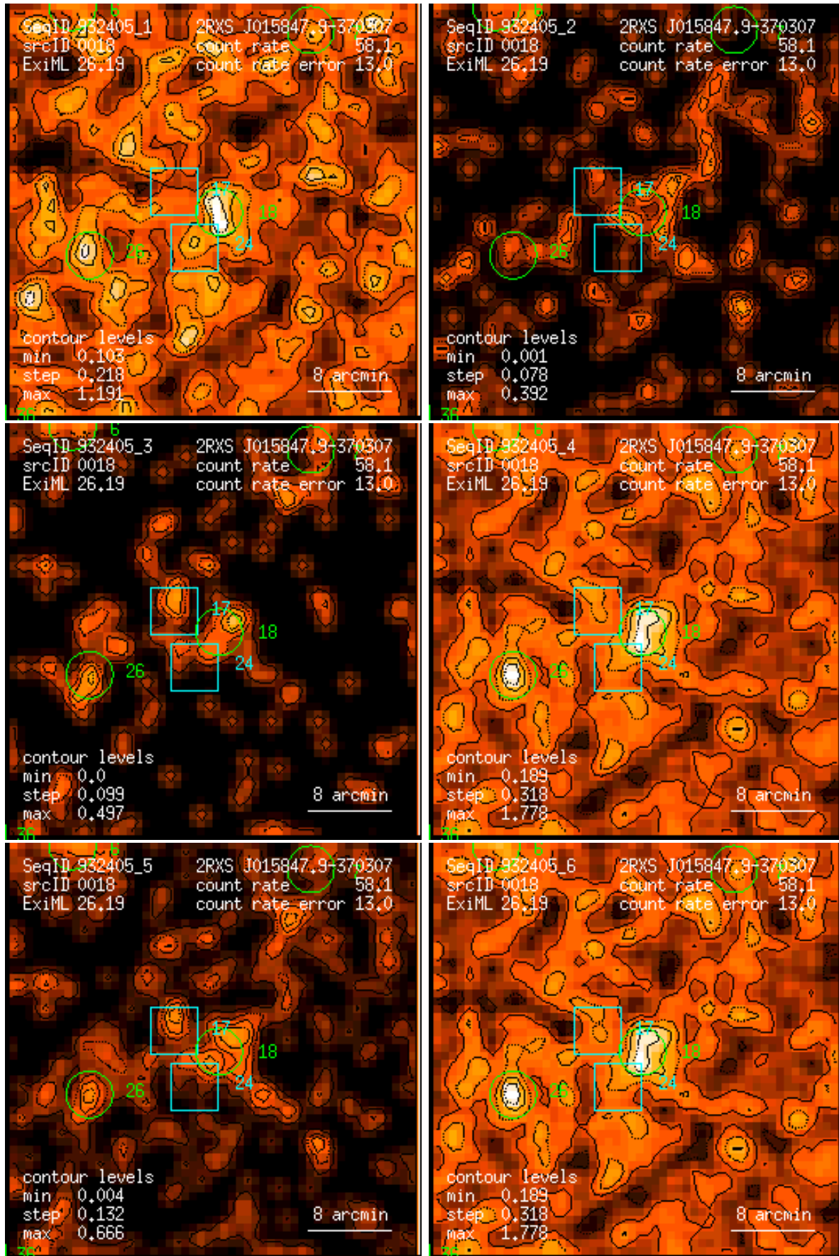
Figure 18: RASS 932405: detection 0018: band rate images, Gaussian filter: (1) PSPC channels 11 – 41, (2) 52 – 90, (3) 91 – 201, (4) 11 – 235, (5) 52 – 201, (6) 11 – 201. Broad band rates in counts/ks. Band rate contour levels in counts/ks/arcmin 2 .
