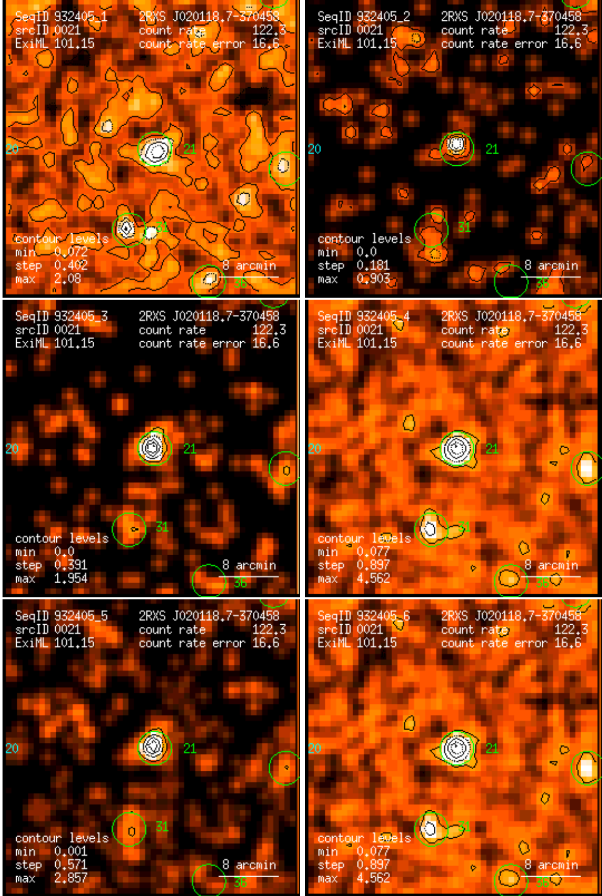
Figure 21: RASS 932405: detection 0021: band rate images, Gaussian filter: (1) PSPC channels 11 – 41, (2) 52 – 90, (3) 91 – 201, (4) 11 – 235, (5) 52 – 201, (6) 11 – 201. Broad band rates in counts/ks. Band rate contour levels in counts/ks/arcmin 2 .
