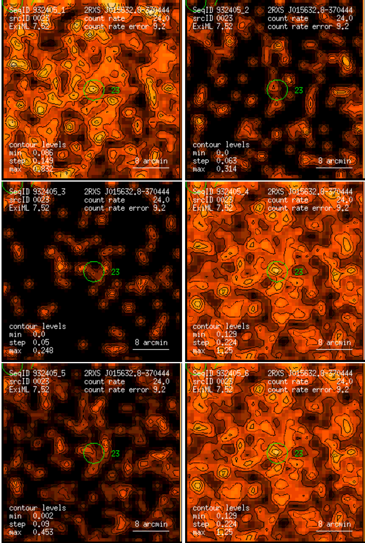
Figure 23: RASS 932405: detection 0023: band rate images, Gaussian filter: (1) PSPC channels 11 – 41, (2) 52 – 90, (3) 91 – 201, (4) 11 – 235, (5) 52 – 201, (6) 11 – 201. Broad band rates in counts/ks. Band rate contour levels in counts/ks/arcmin 2 .
