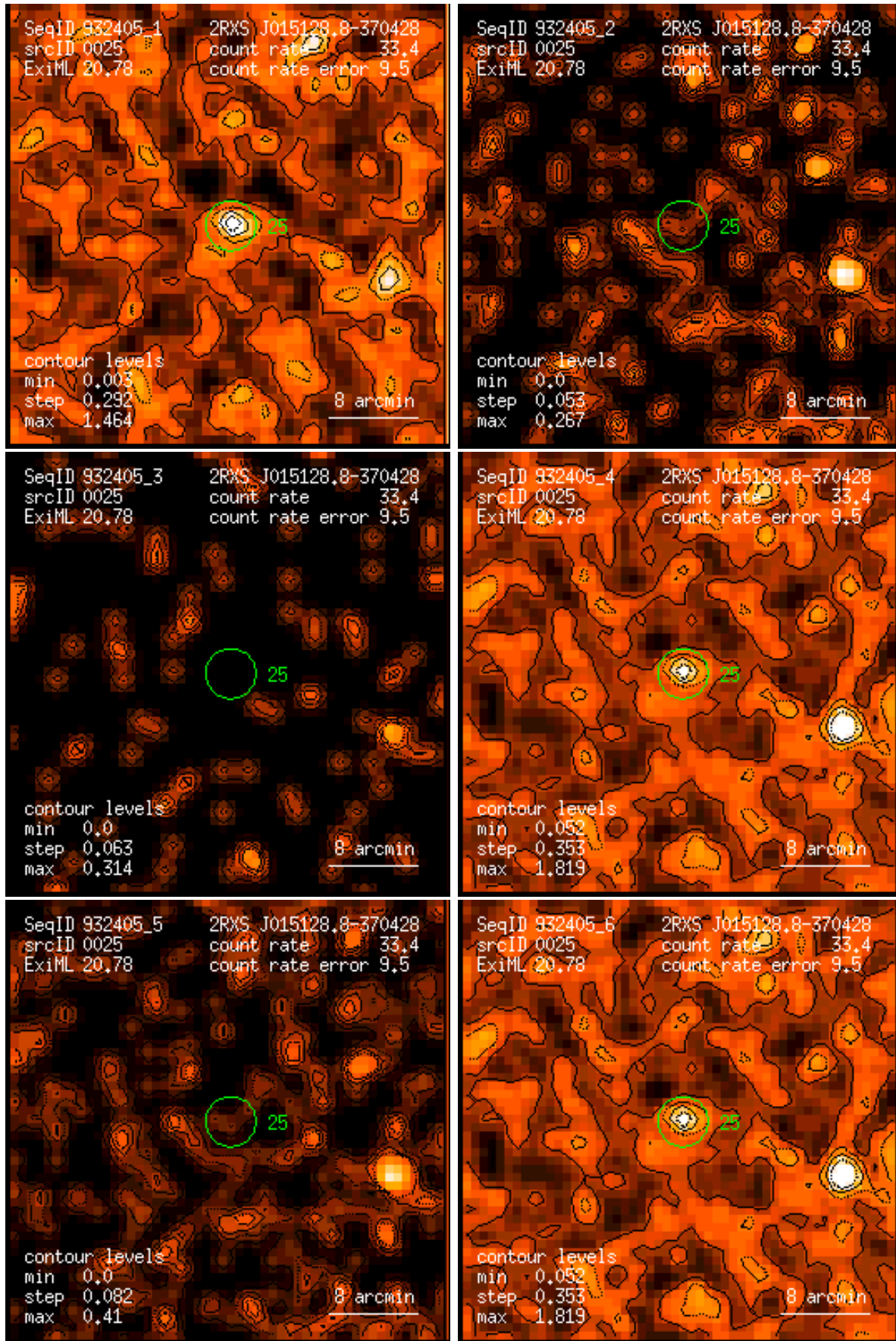
Figure 25: RASS 932405: detection 0025: band rate images, Gaussian filter: (1) PSPC channels 11 – 41, (2) 52 – 90, (3) 91 – 201, (4) 11 – 235, (5) 52 – 201, (6) 11 – 201. Broad band rates in counts/ks. Band rate contour levels in counts/ks/arcmin 2 .
