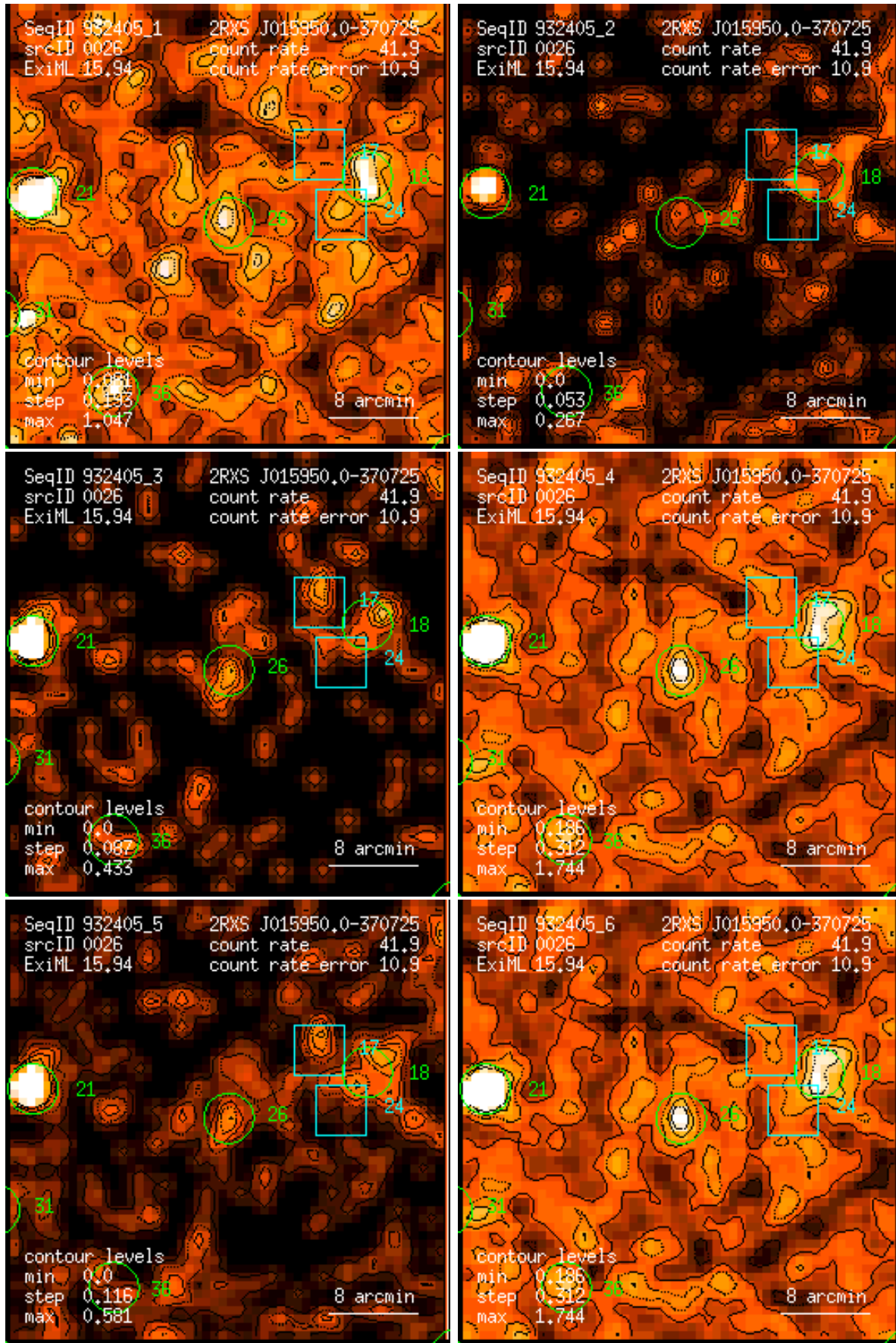
Figure 26: RASS 932405: detection 0026: band rate images, Gaussian filter: (1) PSPC channels 11 – 41, (2) 52 – 90, (3) 91 – 201, (4) 11 – 235, (5) 52 – 201, (6) 11 – 201. Broad band rates in counts/ks. Band rate contour levels in counts/ks/arcmin 2 .
