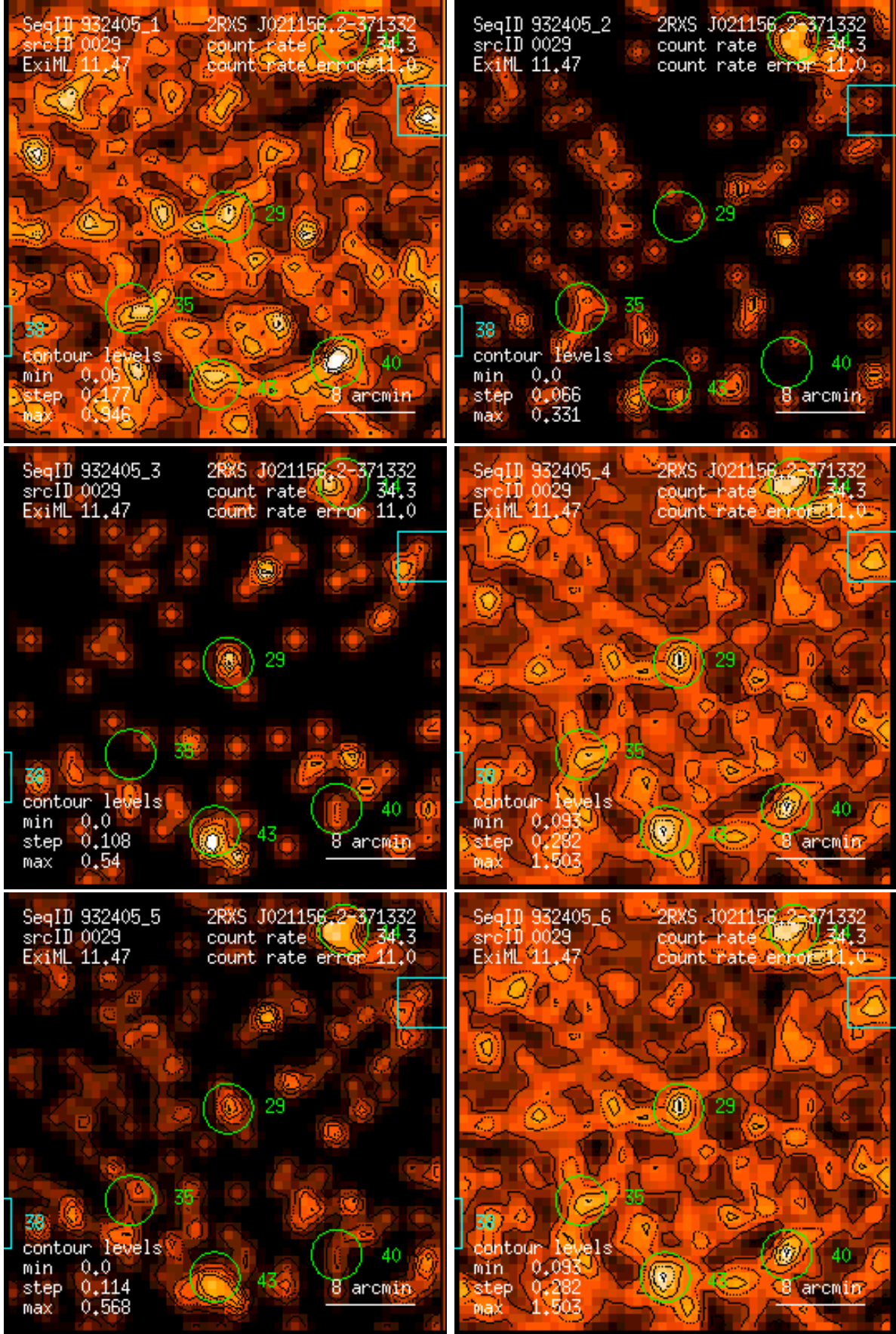
Figure 29: RASS 932405: detection 0029: band rate images, Gaussian filter: (1) PSPC channels 11 – 41, (2) 52 – 90, (3) 91 – 201, (4) 11 – 235, (5) 52 – 201, (6) 11 – 201. Broad band rates in counts/ks. Band rate contour levels in counts/ks/arcmin 2 .
