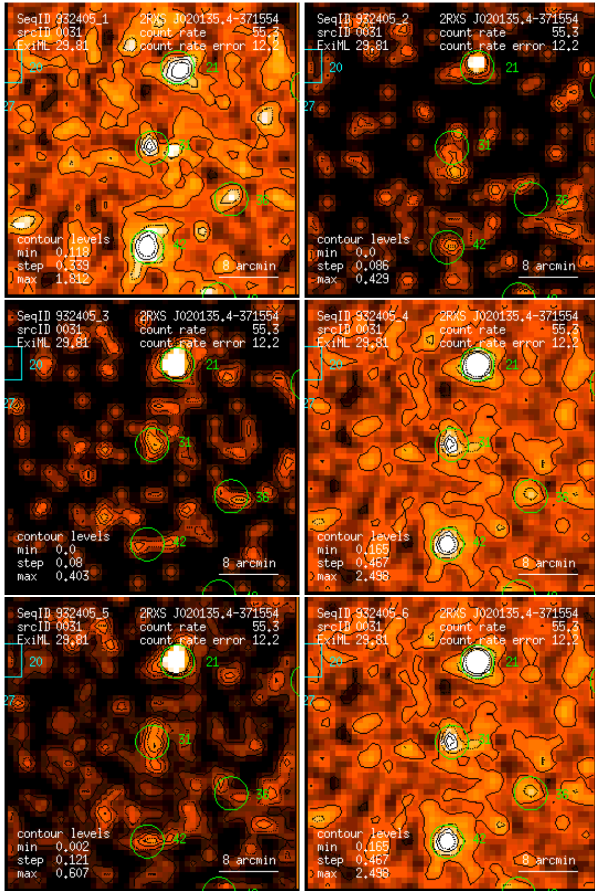
Figure 31: RASS 932405: detection 0031: band rate images, Gaussian filter: (1) PSPC channels 11 – 41, (2) 52 – 90, (3) 91 – 201, (4) 11 – 235, (5) 52 – 201, (6) 11 – 201. Broad band rates in counts/ks. Band rate contour levels in counts/ks/arcmin 2 .
