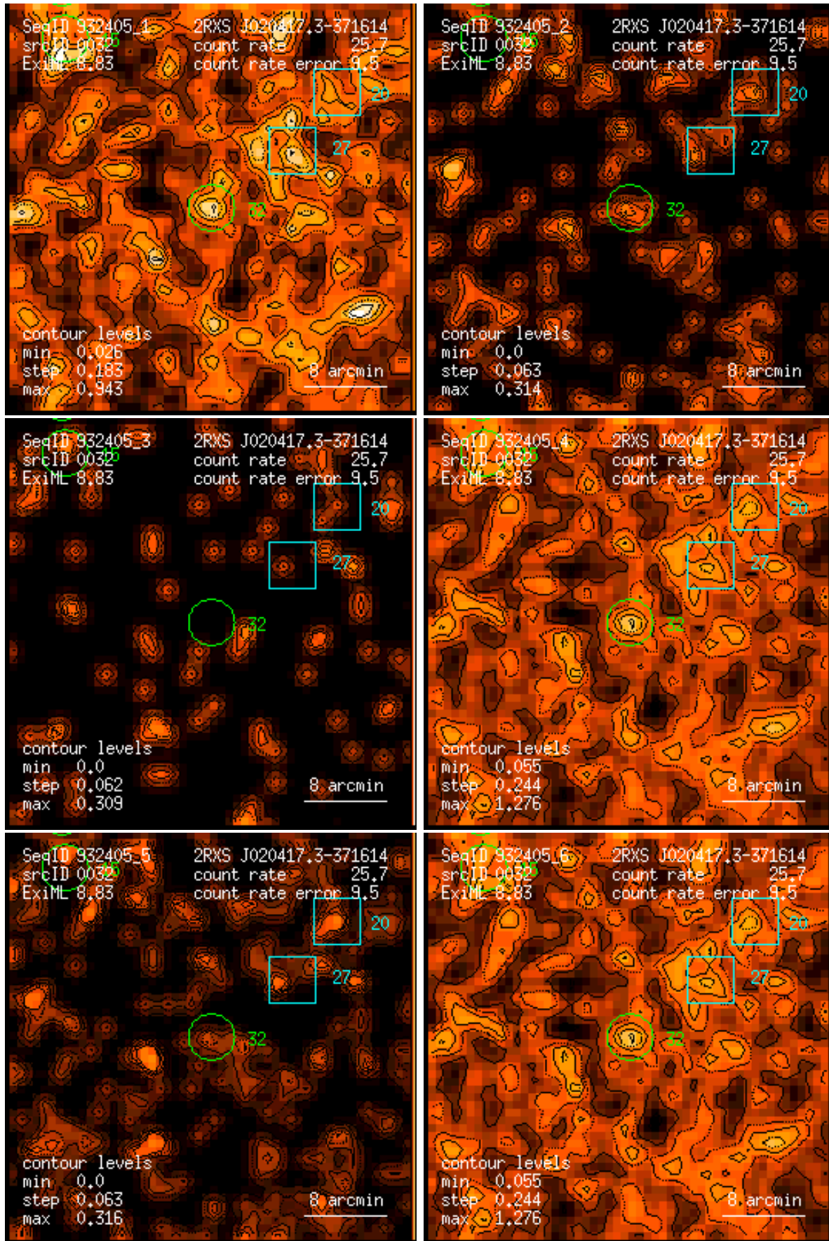
Figure 32: RASS 932405: detection 0032: band rate images, Gaussian filter: (1) PSPC channels 11 – 41, (2) 52 – 90, (3) 91 – 201, (4) 11 – 235, (5) 52 – 201, (6) 11 – 201. Broad band rates in counts/ks. Band rate contour levels in counts/ks/arcmin 2 .
