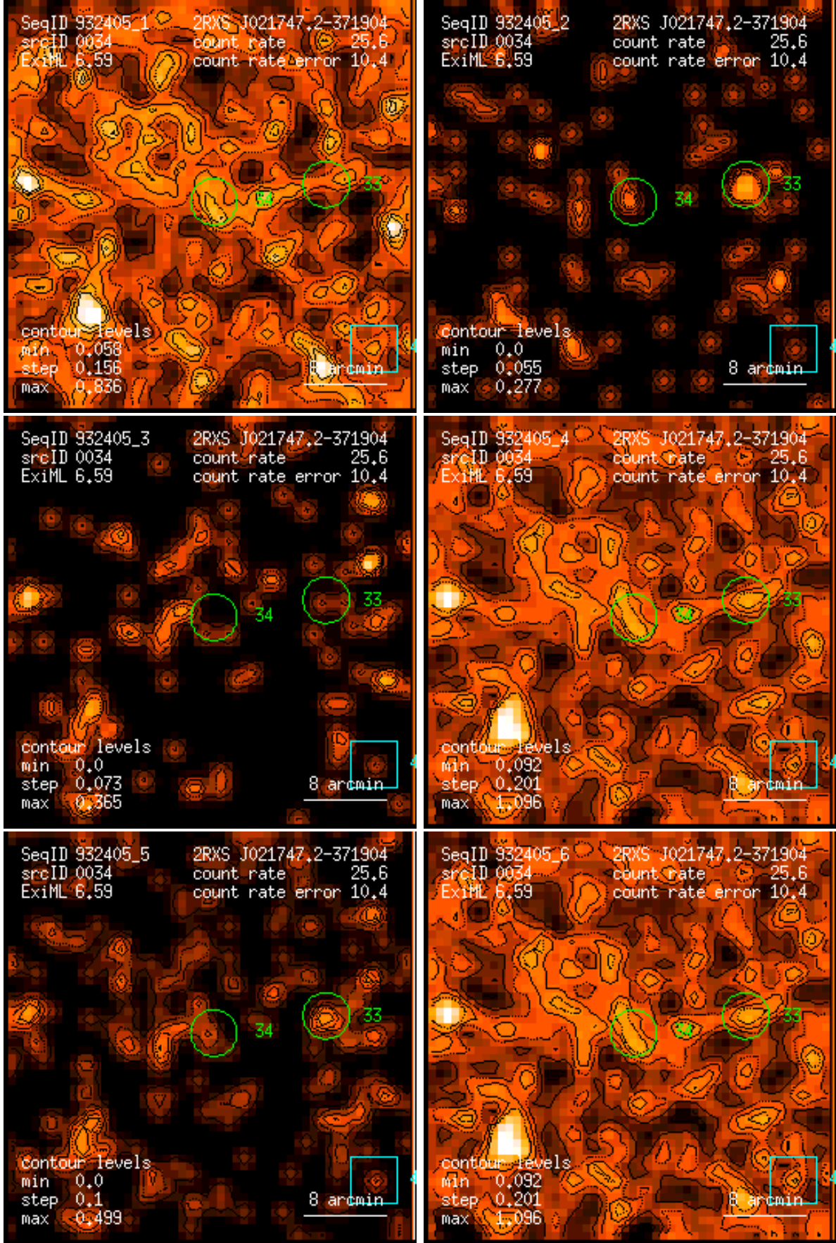
Figure 34: RASS 932405: detection 0034: band rate images, Gaussian filter: (1) PSPC channels 11 – 41, (2) 52 – 90, (3) 91 – 201, (4) 11 – 235, (5) 52 – 201, (6) 11 – 201. Broad band rates in counts/ks. Band rate contour levels in counts/ks/arcmin 2 .
