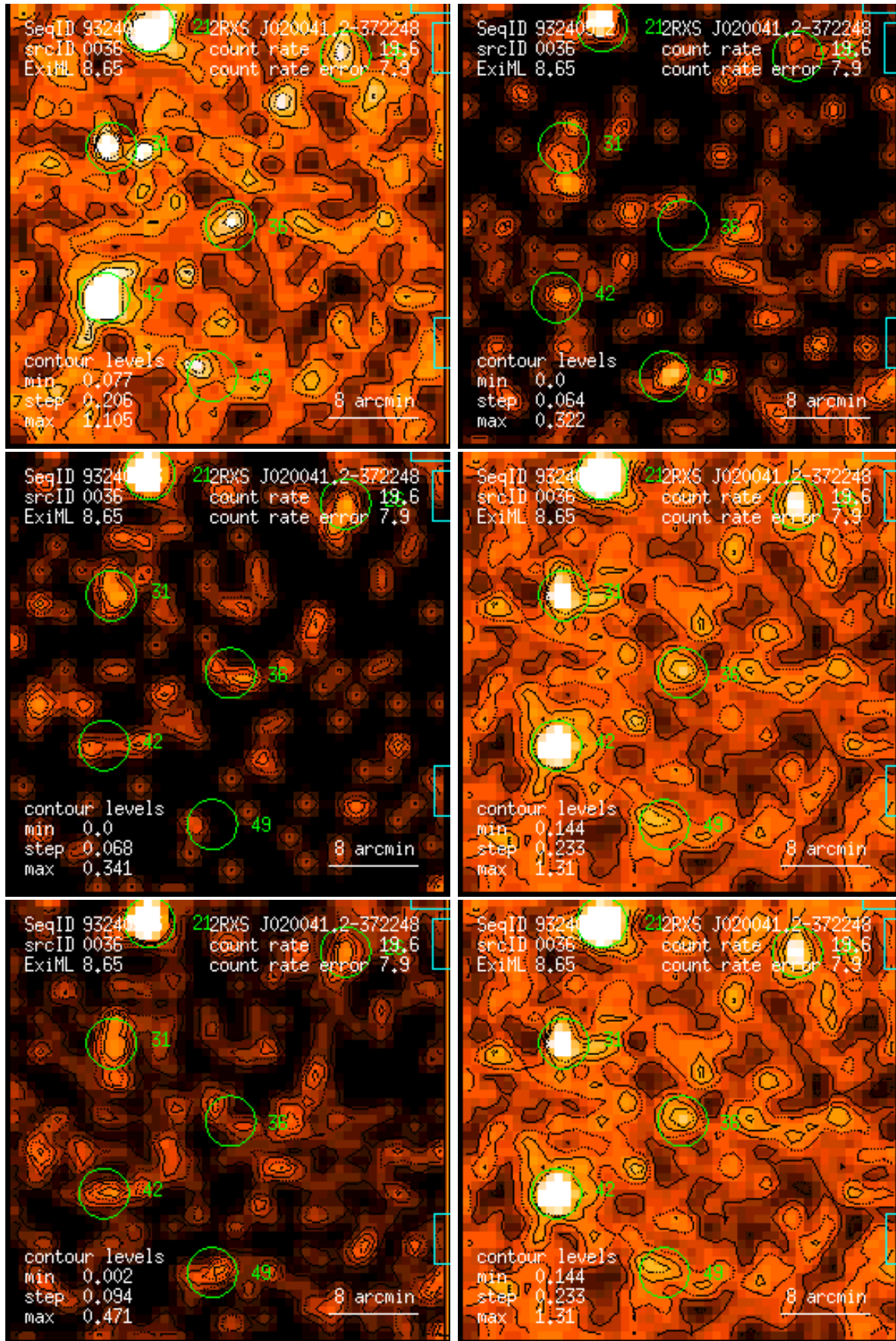
Figure 36: RASS 932405: detection 0036: band rate images, Gaussian filter: (1) PSPC channels 11 – 41, (2) 52 – 90, (3) 91 – 201, (4) 11 – 235, (5) 52 – 201, (6) 11 – 201. Broad band rates in counts/ks. Band rate contour levels in counts/ks/arcmin 2 .
