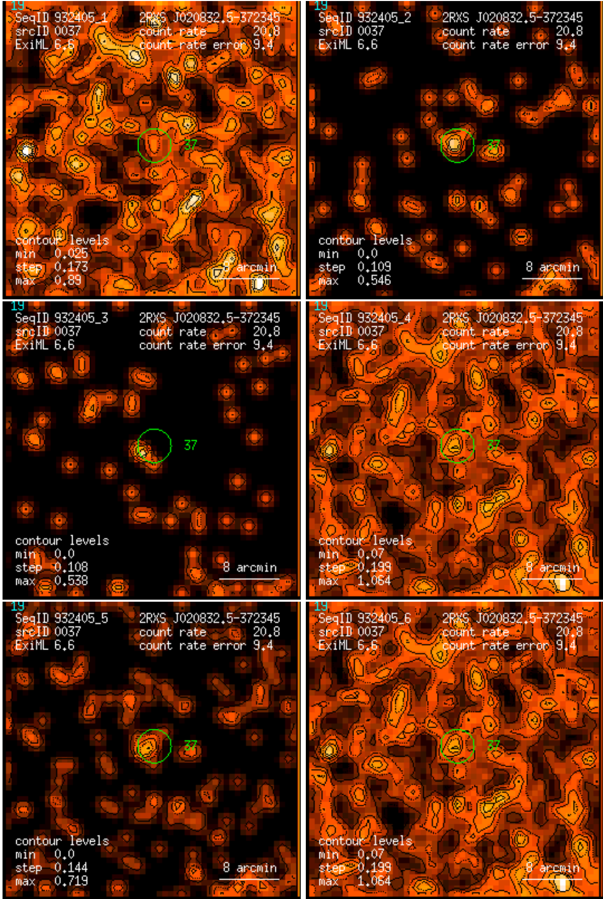
Figure 37: RASS 932405: detection 0037: band rate images, Gaussian filter: (1) PSPC channels 11 – 41, (2) 52 – 90, (3) 91 – 201, (4) 11 – 235, (5) 52 – 201, (6) 11 – 201. Broad band rates in counts/ks. Band rate contour levels in counts/ks/arcmin 2 .
