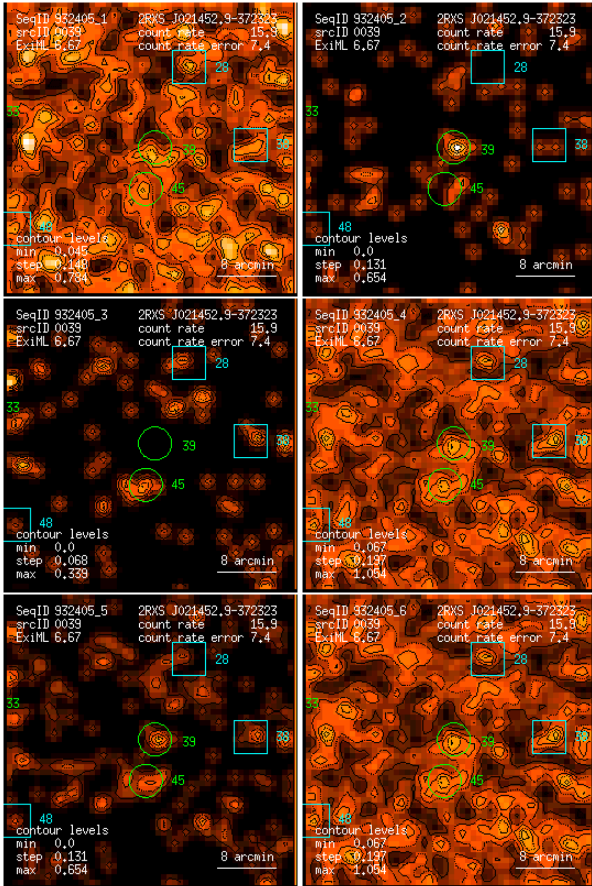
Figure 39: RASS 932405: detection 0039: band rate images, Gaussian filter: (1) PSPC channels 11 – 41, (2) 52 – 90, (3) 91 – 201, (4) 11 – 235, (5) 52 – 201, (6) 11 – 201. Broad band rates in counts/ks. Band rate contour levels in counts/ks/arcmin 2 .
