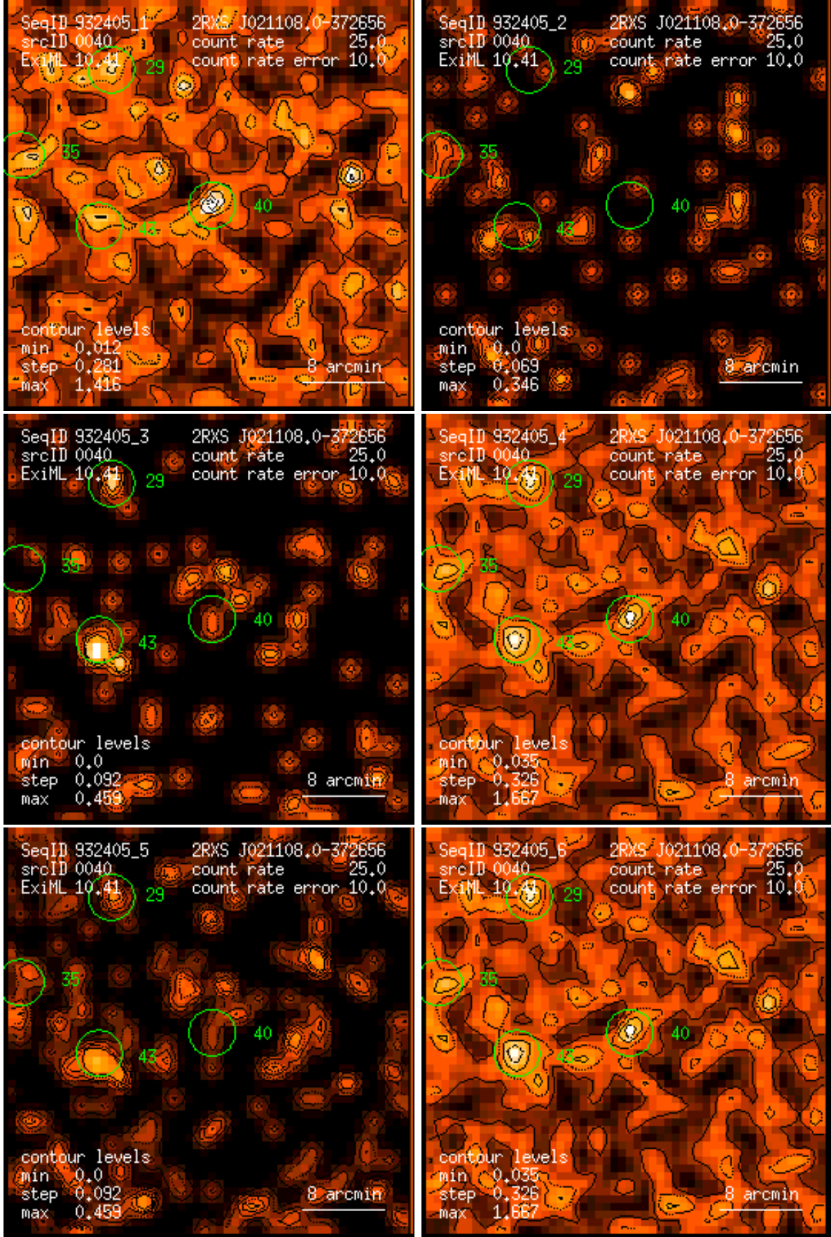
Figure 40: RASS 932405: detection 0040: band rate images, Gaussian filter: (1) PSPC channels 11 – 41, (2) 52 – 90, (3) 91 – 201, (4) 11 – 235, (5) 52 – 201, (6) 11 – 201. Broad band rates in counts/ks. Band rate contour levels in counts/ks/arcmin 2 .
