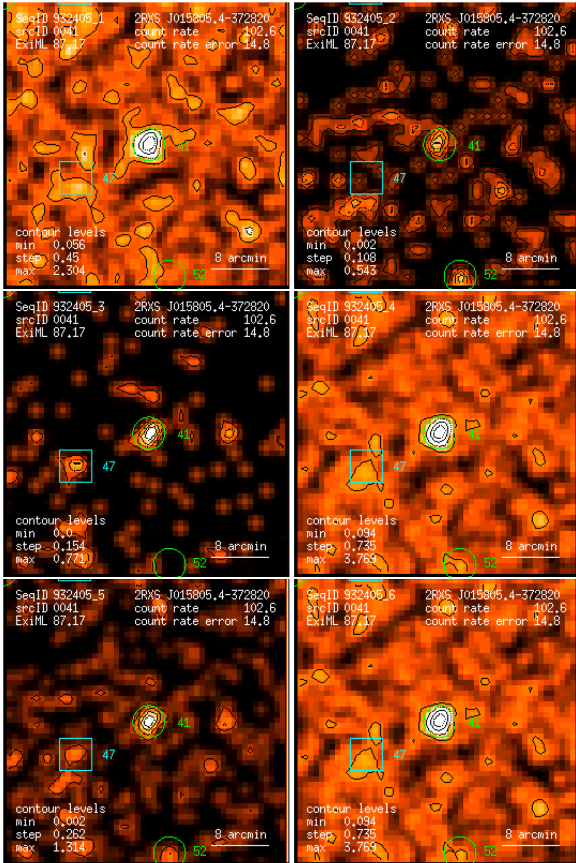
Figure 41: RASS 932405: detection 0041: band rate images, Gaussian filter: (1) PSPC channels 11 – 41, (2) 52 – 90, (3) 91 – 201, (4) 11 – 235, (5) 52 – 201, (6) 11 – 201. Broad band rates in counts/ks. Band rate contour levels in counts/ks/arcmin 2 .
