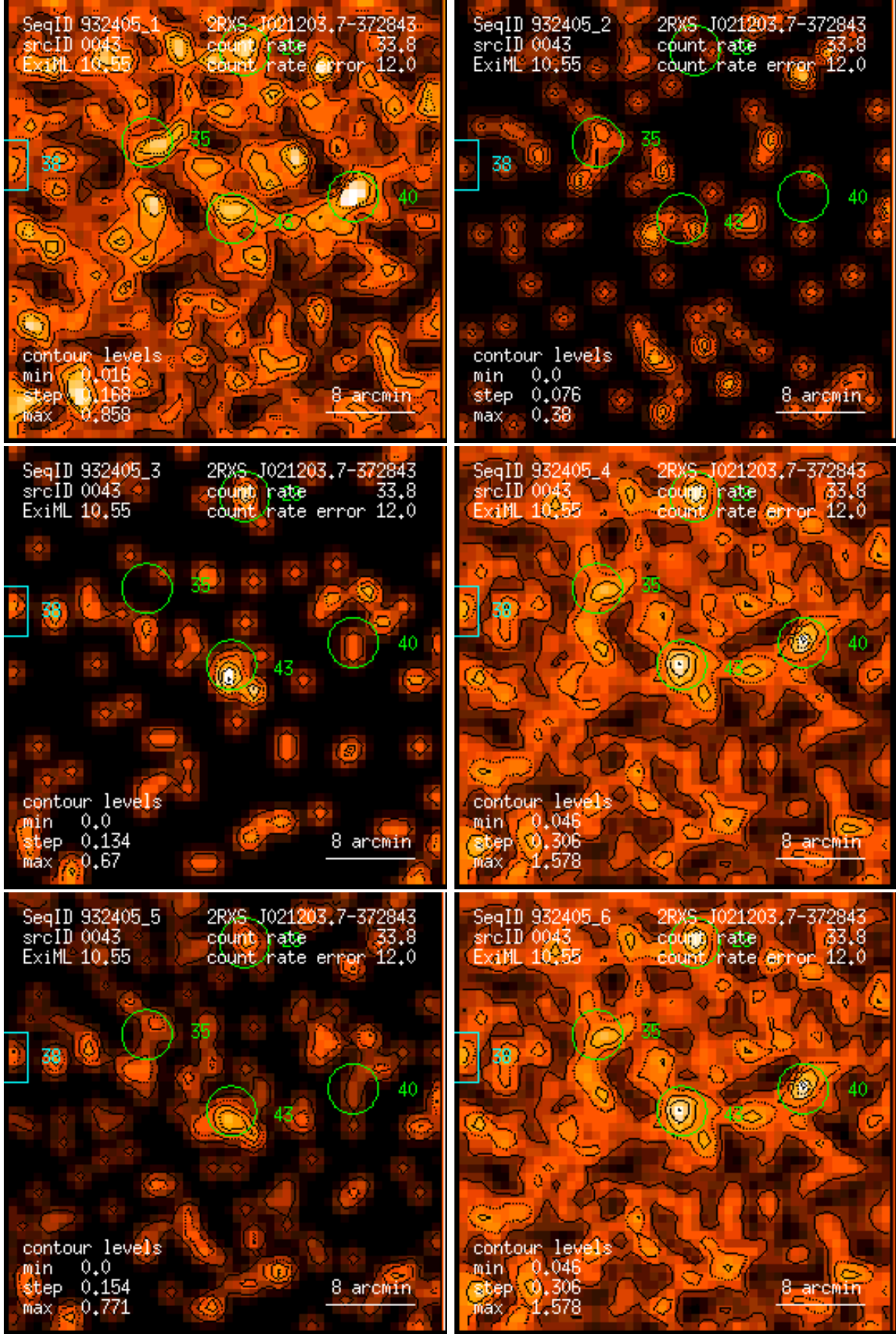
Figure 43: RASS 932405: detection 0043: band rate images, Gaussian filter: (1) PSPC channels 11 – 41, (2) 52 – 90, (3) 91 – 201, (4) 11 – 235, (5) 52 – 201, (6) 11 – 201. Broad band rates in counts/ks. Band rate contour levels in counts/ks/arcmin 2 .
