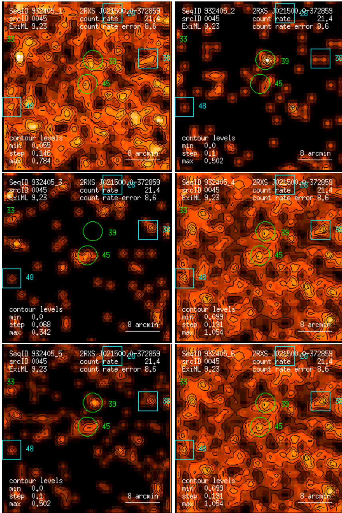
Figure 45: RASS 932405: detection 0045: band rate images, Gaussian filter: (1) PSPC channels 11 – 41, (2) 52 – 90, (3) 91 – 201, (4) 11 – 235, (5) 52 – 201, (6) 11 – 201. Broad band rates in counts/ks. Band rate contour levels in counts/ks/arcmin 2 .
