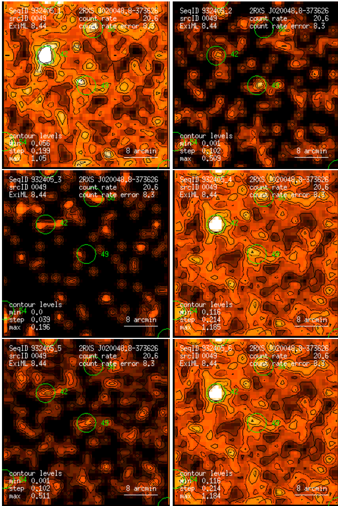
Figure 49: RASS 932405: detection 0049: band rate images, Gaussian filter: (1) PSPC channels 11 – 41, (2) 52 – 90, (3) 91 – 201, (4) 11 – 235, (5) 52 – 201, (6) 11 – 201. Broad band rates in counts/ks. Band rate contour levels in counts/ks/arcmin 2 .
