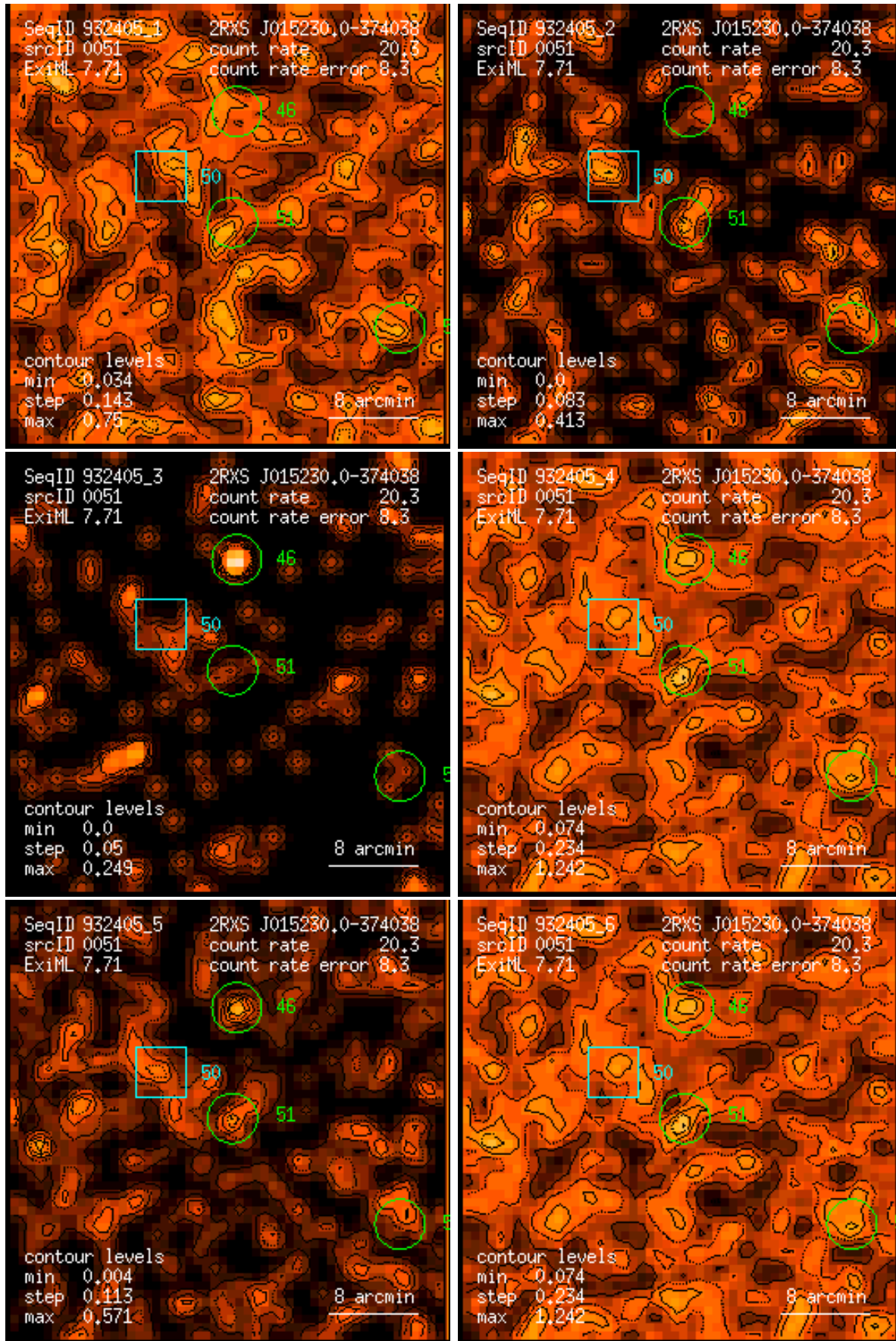
Figure 51: RASS 932405: detection 0051: band rate images, Gaussian filter: (1) PSPC channels 11 – 41, (2) 52 – 90, (3) 91 – 201, (4) 11 – 235, (5) 52 – 201, (6) 11 – 201. Broad band rates in counts/ks. Band rate contour levels in counts/ks/arcmin 2 .
