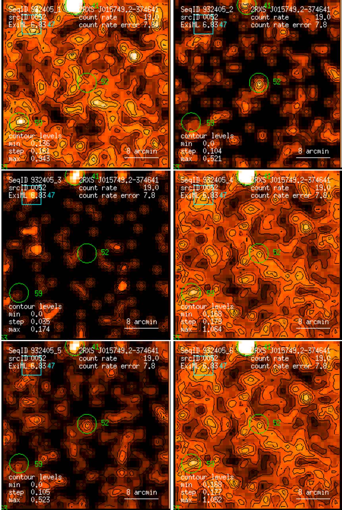
Figure 52: RASS 932405: detection 0052: band rate images, Gaussian filter: (1) PSPC channels 11 – 41, (2) 52 – 90, (3) 91 – 201, (4) 11 – 235, (5) 52 – 201, (6) 11 – 201. Broad band rates in counts/ks. Band rate contour levels in counts/ks/arcmin 2 .
