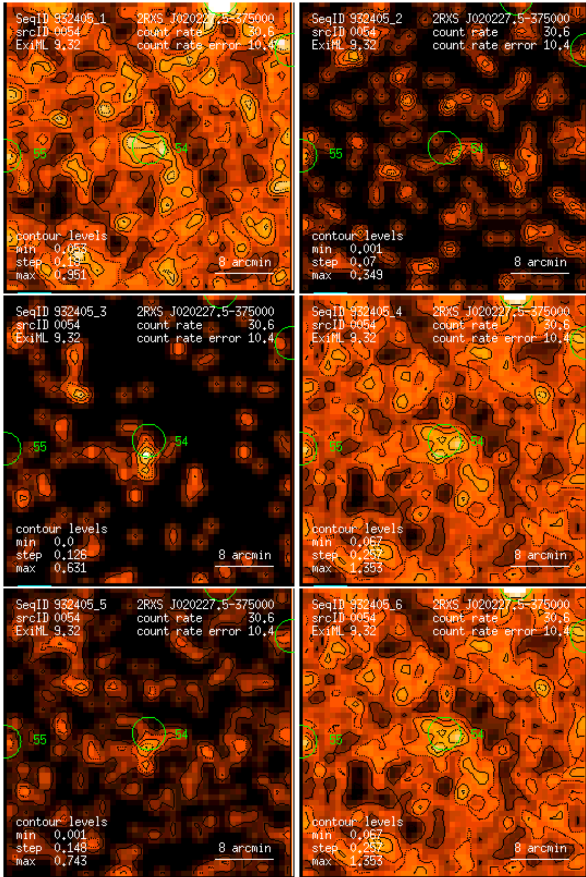
Figure 54: RASS 932405: detection 0054: band rate images, Gaussian filter: (1) PSPC channels 11 – 41, (2) 52 – 90, (3) 91 – 201, (4) 11 – 235, (5) 52 – 201, (6) 11 – 201. Broad band rates in counts/ks. Band rate contour levels in counts/ks/arcmin 2 .
