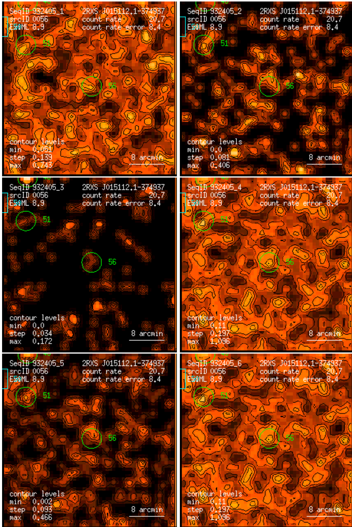
Figure 56: RASS 932405: detection 0056: band rate images, Gaussian filter: (1) PSPC channels 11 – 41, (2) 52 – 90, (3) 91 – 201, (4) 11 – 235, (5) 52 – 201, (6) 11 – 201. Broad band rates in counts/ks. Band rate contour levels in counts/ks/arcmin 2 .
