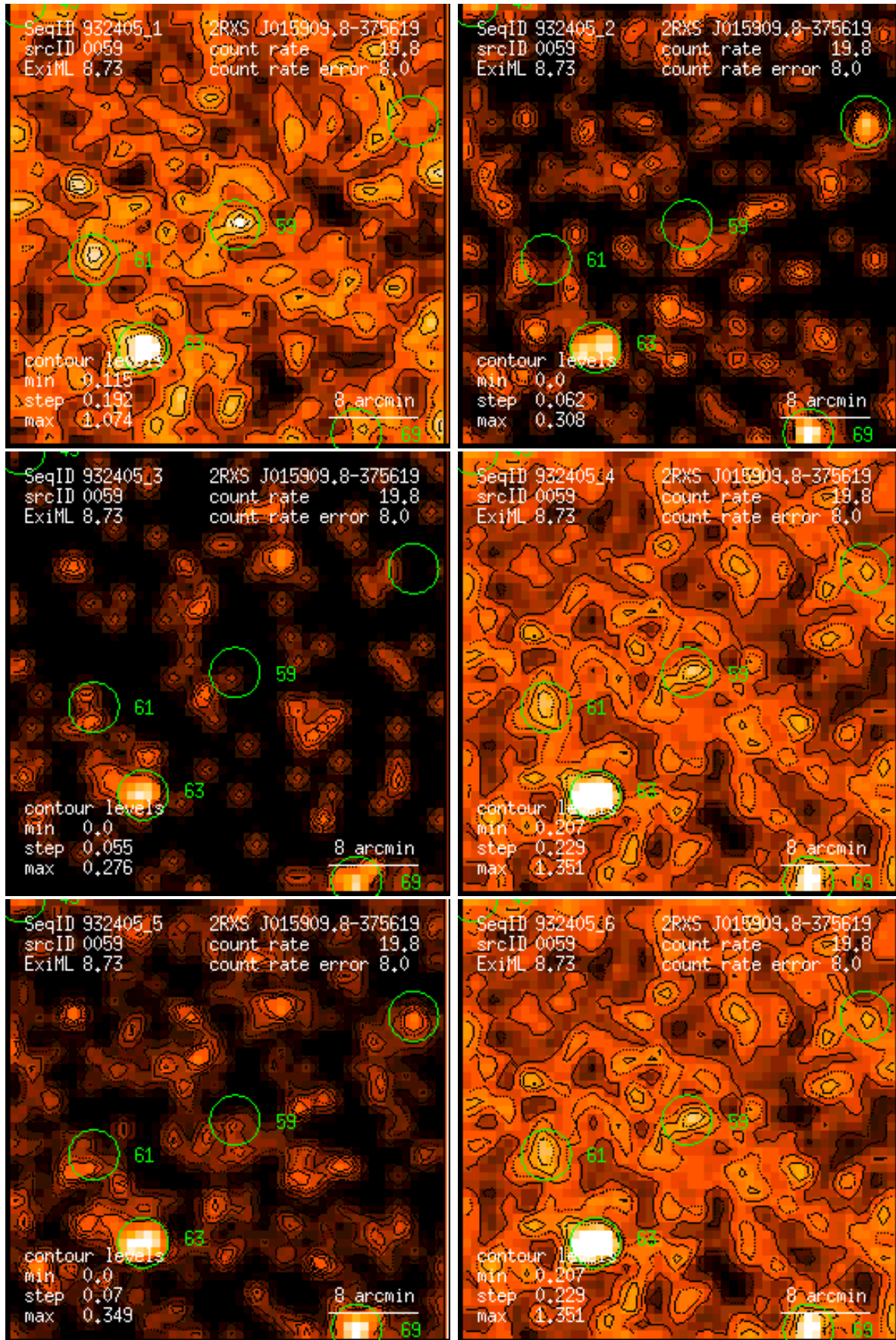
Figure 59: RASS 932405: detection 0059: band rate images, Gaussian filter: (1) PSPC channels 11 – 41, (2) 52 – 90, (3) 91 – 201, (4) 11 – 235, (5) 52 – 201, (6) 11 – 201. Broad band rates in counts/ks. Band rate contour levels in counts/ks/arcmin 2 .
