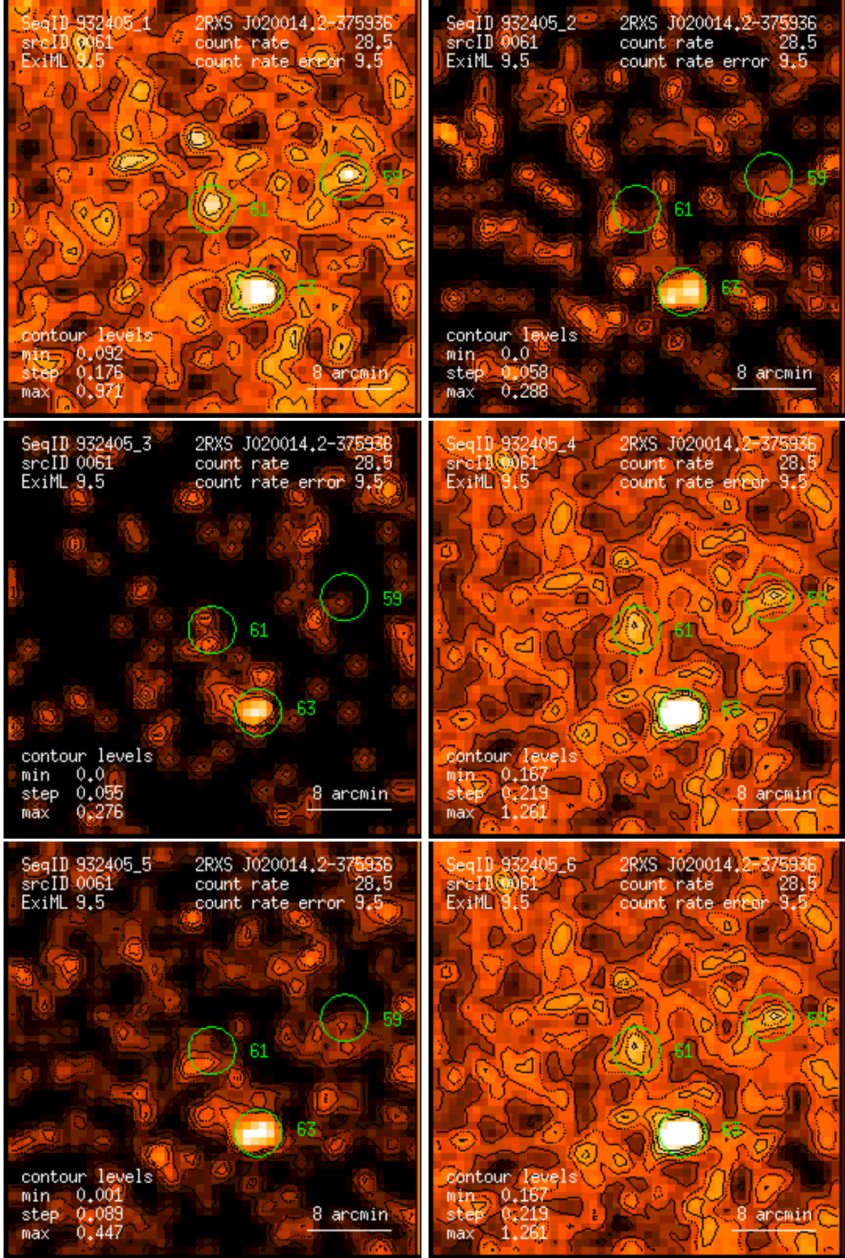
Figure 61: RASS 932405: detection 0061: band rate images, Gaussian filter: (1) PSPC channels 11 – 41, (2) 52 – 90, (3) 91 – 201, (4) 11 – 235, (5) 52 – 201, (6) 11 – 201. Broad band rates in counts/ks. Band rate contour levels in counts/ks/arcmin 2 .
