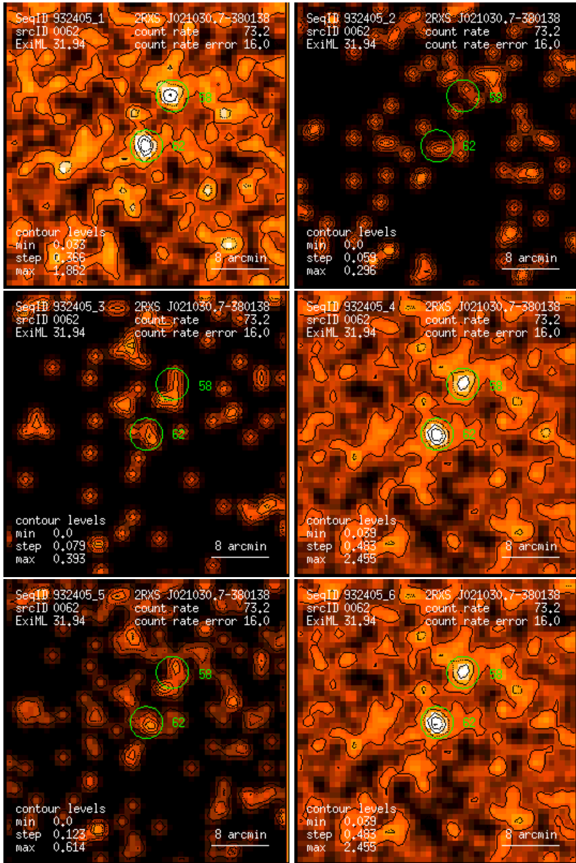
Figure 62: RASS 932405: detection 0062: band rate images, Gaussian filter: (1) PSPC channels 11 – 41, (2) 52 – 90, (3) 91 – 201, (4) 11 – 235, (5) 52 – 201, (6) 11 – 201. Broad band rates in counts/ks. Band rate contour levels in counts/ks/arcmin 2 .
