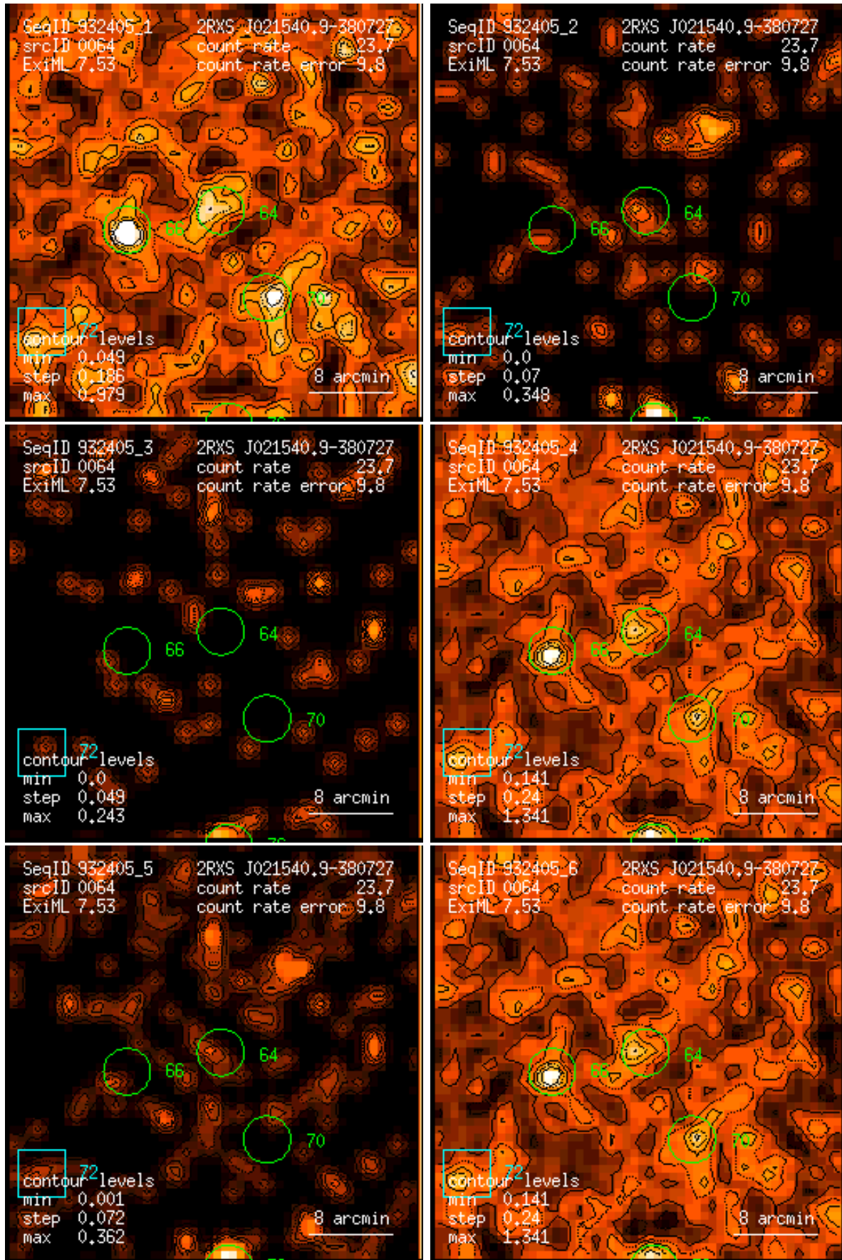
Figure 64: RASS 932405: detection 0064: band rate images, Gaussian filter: (1) PSPC channels 11 – 41, (2) 52 – 90, (3) 91 – 201, (4) 11 – 235, (5) 52 – 201, (6) 11 – 201. Broad band rates in counts/ks. Band rate contour levels in counts/ks/arcmin 2 .
