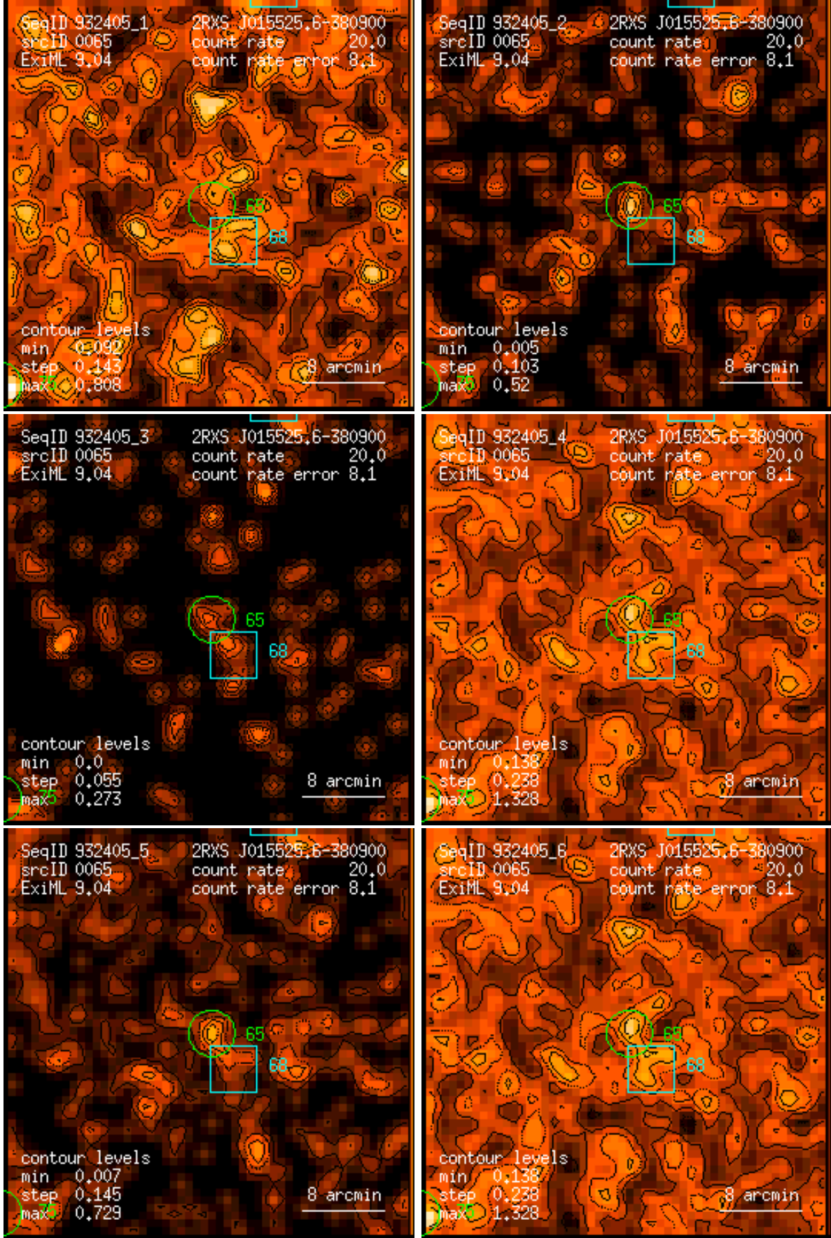
Figure 65: RASS 932405: detection 0065: band rate images, Gaussian filter: (1) PSPC channels 11 – 41, (2) 52 – 90, (3) 91 – 201, (4) 11 – 235, (5) 52 – 201, (6) 11 – 201. Broad band rates in counts/ks. Band rate contour levels in counts/ks/arcmin 2 .
