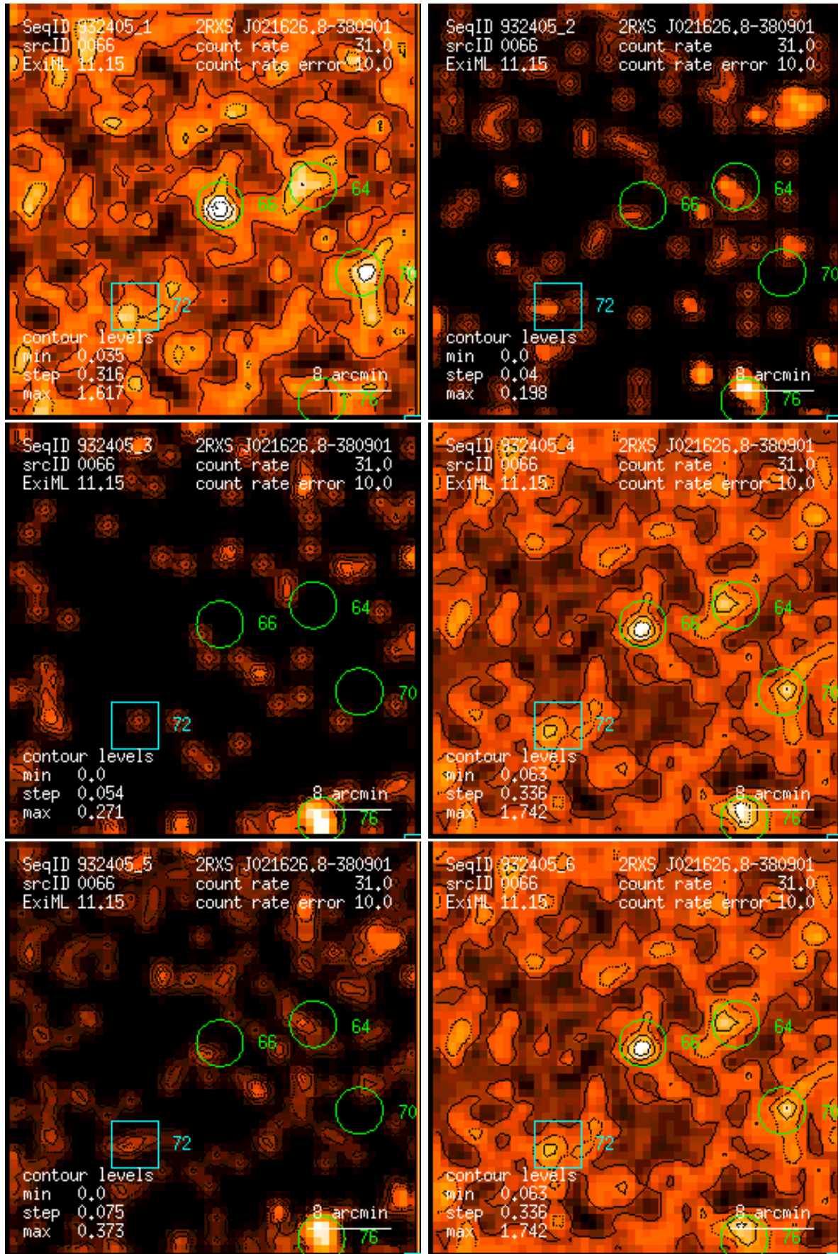
Figure 66: RASS 932405: detection 0066: band rate images, Gaussian filter: (1) PSPC channels 11 – 41, (2) 52 – 90, (3) 91 – 201, (4) 11 – 235, (5) 52 – 201, (6) 11 – 201. Broad band rates in counts/ks. Band rate contour levels in counts/ks/arcmin 2 .
