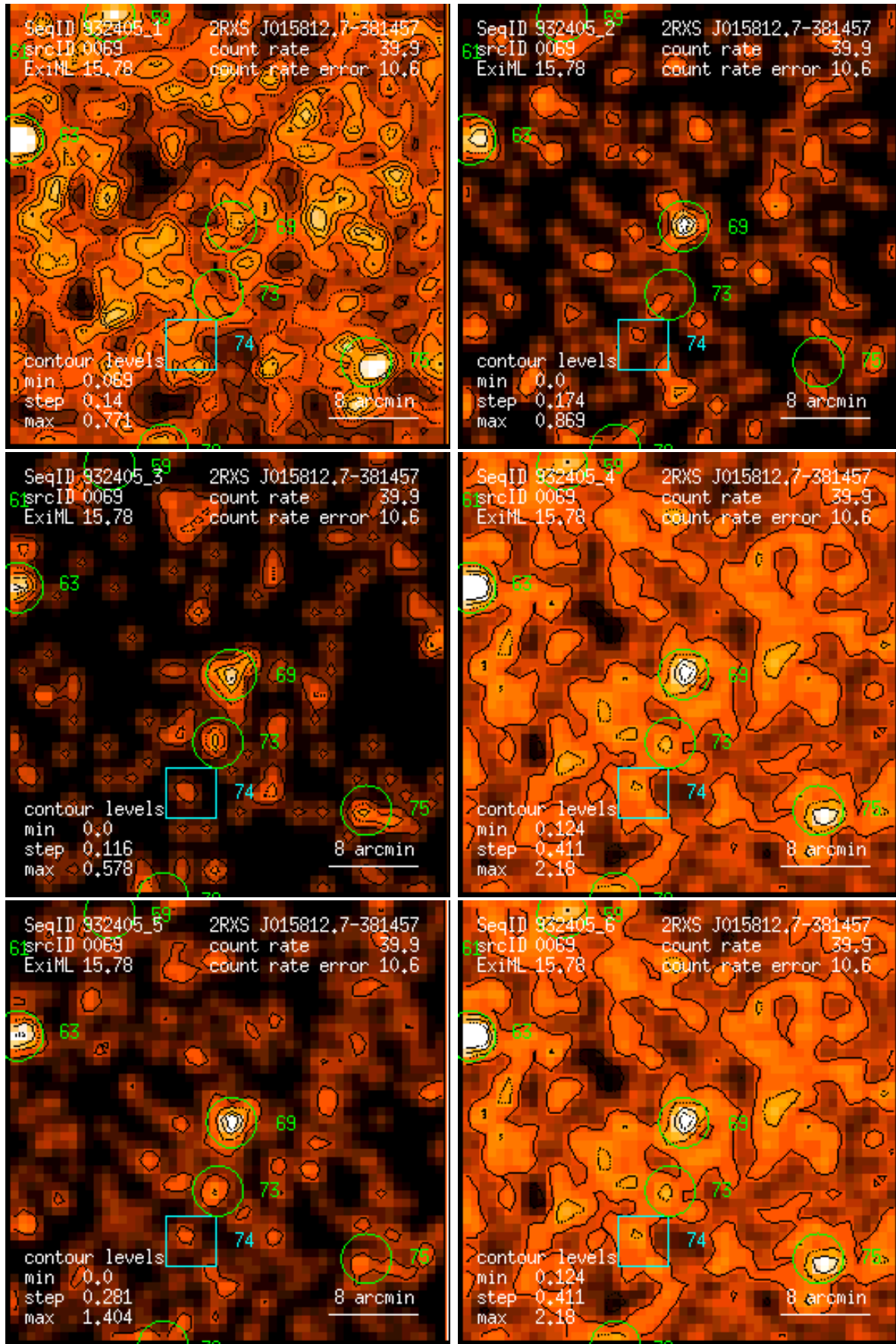
Figure 69: RASS 932405: detection 0069: band rate images, Gaussian filter: (1) PSPC channels 11 – 41, (2) 52 – 90, (3) 91 – 201, (4) 11 – 235, (5) 52 – 201, (6) 11 – 201. Broad band rates in counts/ks. Band rate contour levels in counts/ks/arcmin 2 .
