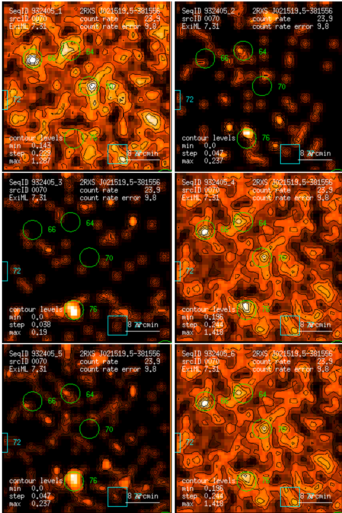
Figure 70: RASS 932405: detection 0070: band rate images, Gaussian filter: (1) PSPC channels 11 – 41, (2) 52 – 90, (3) 91 – 201, (4) 11 – 235, (5) 52 – 201, (6) 11 – 201. Broad band rates in counts/ks. Band rate contour levels in counts/ks/arcmin 2 .
