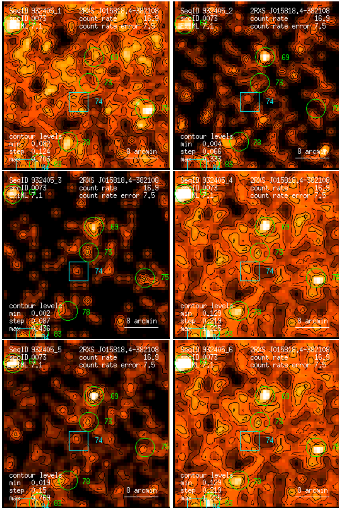
Figure 73: RASS 932405: detection 0073: band rate images, Gaussian filter: (1) PSPC channels 11 – 41, (2) 52 – 90, (3) 91 – 201, (4) 11 – 235, (5) 52 – 201, (6) 11 – 201. Broad band rates in counts/ks. Band rate contour levels in counts/ks/arcmin 2 .
