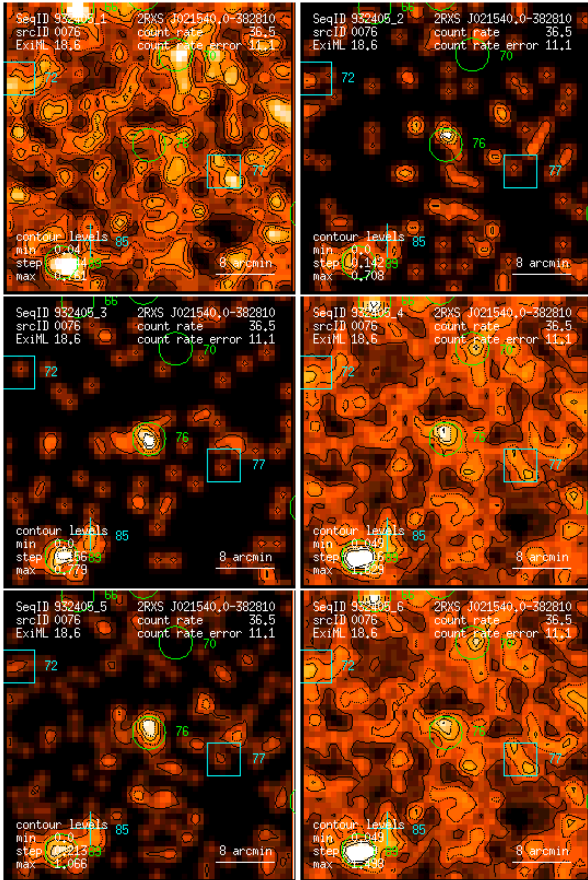
Figure 76: RASS 932405: detection 0076: band rate images, Gaussian filter: (1) PSPC channels 11 – 41, (2) 52 – 90, (3) 91 – 201, (4) 11 – 235, (5) 52 – 201, (6) 11 – 201. Broad band rates in counts/ks. Band rate contour levels in counts/ks/arcmin 2 .
