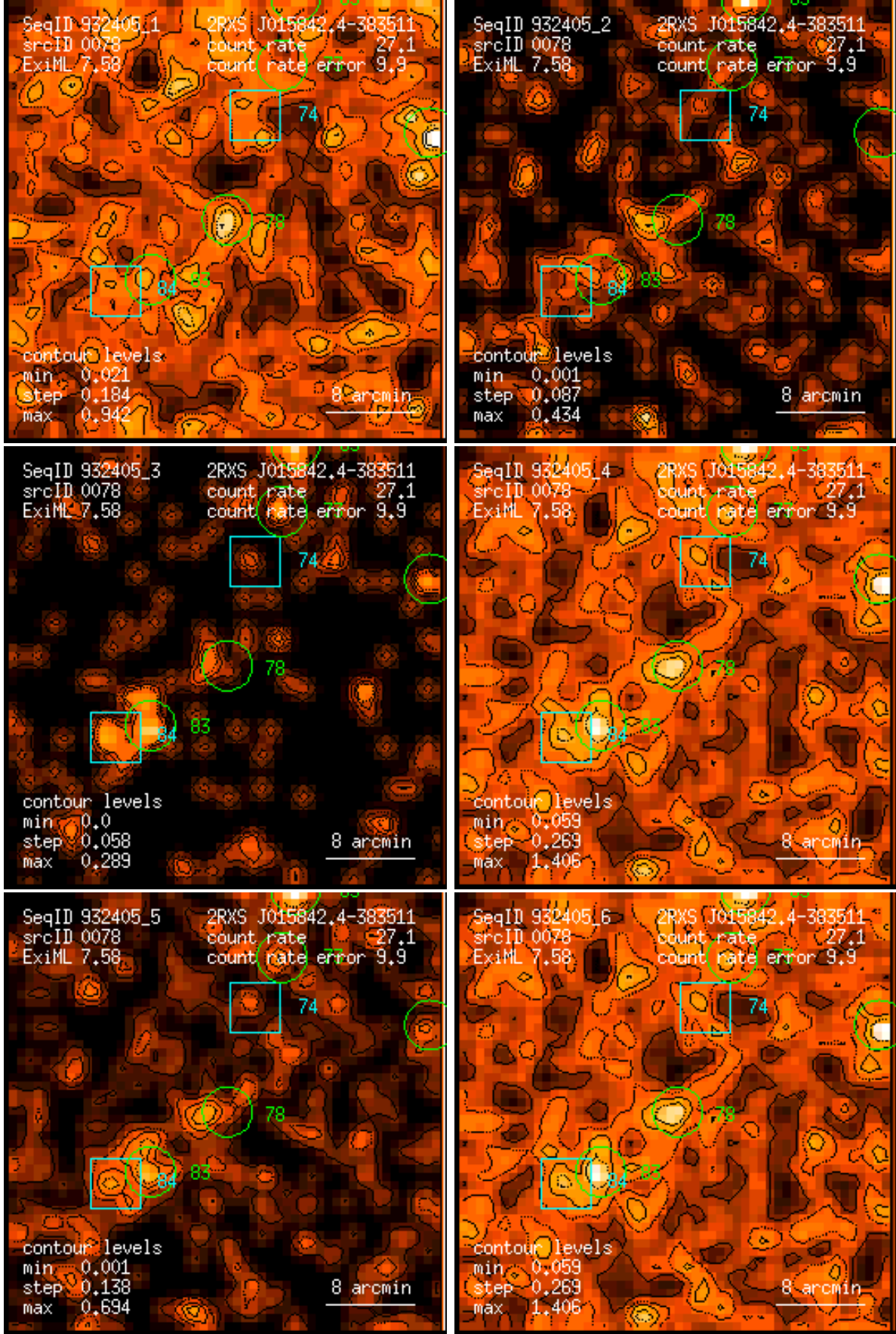
Figure 78: RASS 932405: detection 0078: band rate images, Gaussian filter: (1) PSPC channels 11 – 41, (2) 52 – 90, (3) 91 – 201, (4) 11 – 235, (5) 52 – 201, (6) 11 – 201. Broad band rates in counts/ks. Band rate contour levels in counts/ks/arcmin 2 .
