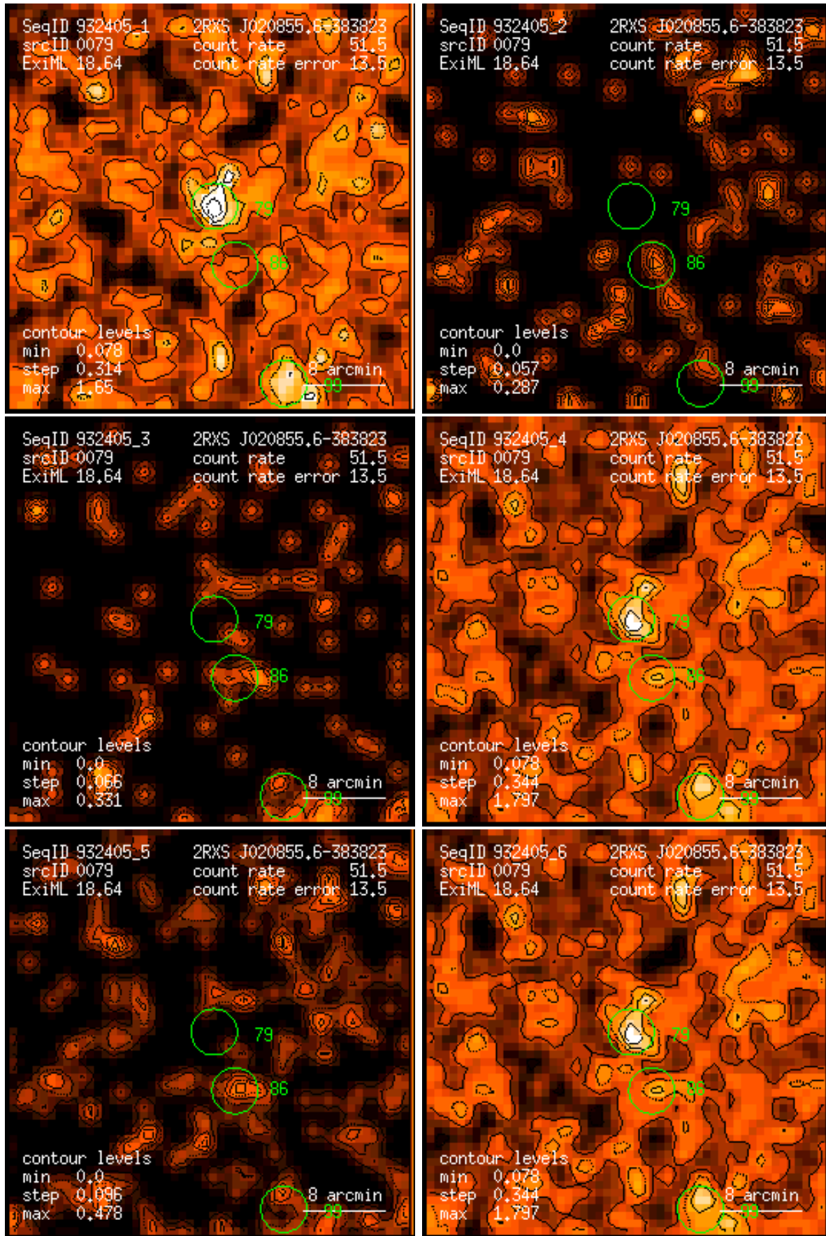
Figure 79: RASS 932405: detection 0079: band rate images, Gaussian filter: (1) PSPC channels 11 – 41, (2) 52 – 90, (3) 91 – 201, (4) 11 – 235, (5) 52 – 201, (6) 11 – 201. Broad band rates in counts/ks. Band rate contour levels in counts/ks/arcmin 2 .
