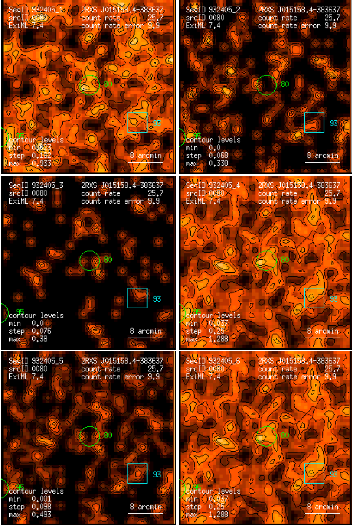
Figure 80: RASS 932405: detection 0080: band rate images, Gaussian filter: (1) PSPC channels 11 – 41, (2) 52 – 90, (3) 91 – 201, (4) 11 – 235, (5) 52 – 201, (6) 11 – 201. Broad band rates in counts/ks. Band rate contour levels in counts/ks/arcmin 2 .
