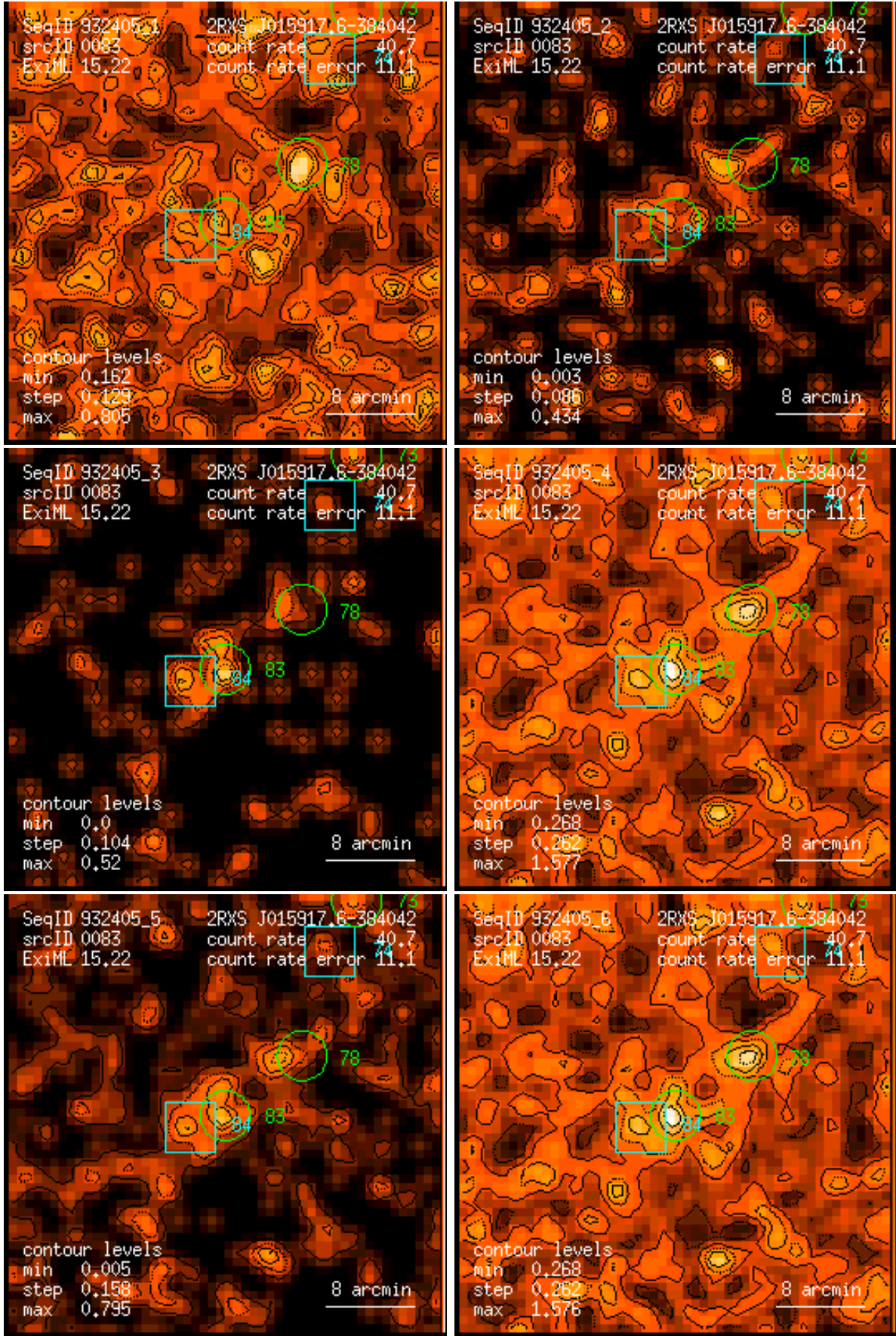
Figure 83: RASS 932405: detection 0083: band rate images, Gaussian filter: (1) PSPC channels 11 – 41, (2) 52 – 90, (3) 91 – 201, (4) 11 – 235, (5) 52 – 201, (6) 11 – 201. Broad band rates in counts/ks. Band rate contour levels in counts/ks/arcmin 2 .
