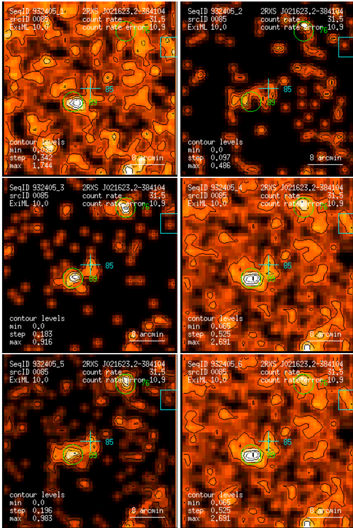
Figure 85: RASS 932405: detection 0085: band rate images, Gaussian filter: (1) PSPC channels 11 – 41, (2) 52 – 90, (3) 91 – 201, (4) 11 – 235, (5) 52 – 201, (6) 11 – 201. Broad band rates in counts/ks. Band rate contour levels in counts/ks/arcmin 2 .
