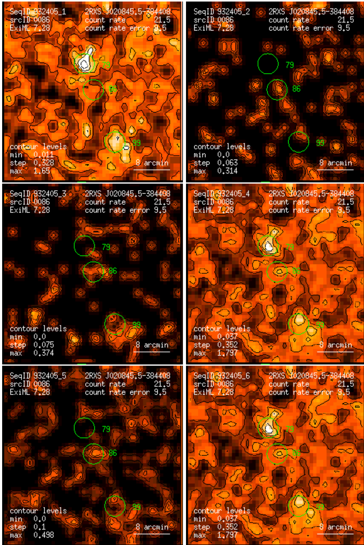
Figure 86: RASS 932405: detection 0086: band rate images, Gaussian filter: (1) PSPC channels 11 – 41, (2) 52 – 90, (3) 91 – 201, (4) 11 – 235, (5) 52 – 201, (6) 11 – 201. Broad band rates in counts/ks. Band rate contour levels in counts/ks/arcmin 2 .
