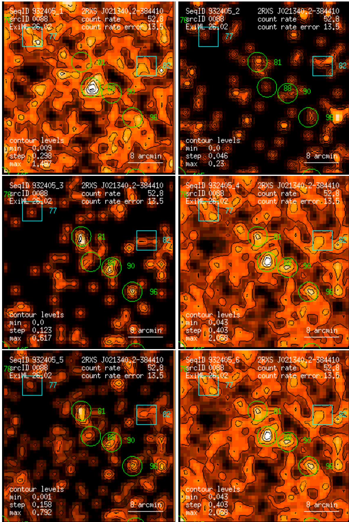
Figure 88: RASS 932405: detection 0088: band rate images, Gaussian filter: (1) PSPC channels 11 – 41, (2) 52 – 90, (3) 91 – 201, (4) 11 – 235, (5) 52 – 201, (6) 11 – 201. Broad band rates in counts/ks. Band rate contour levels in counts/ks/arcmin 2 .
