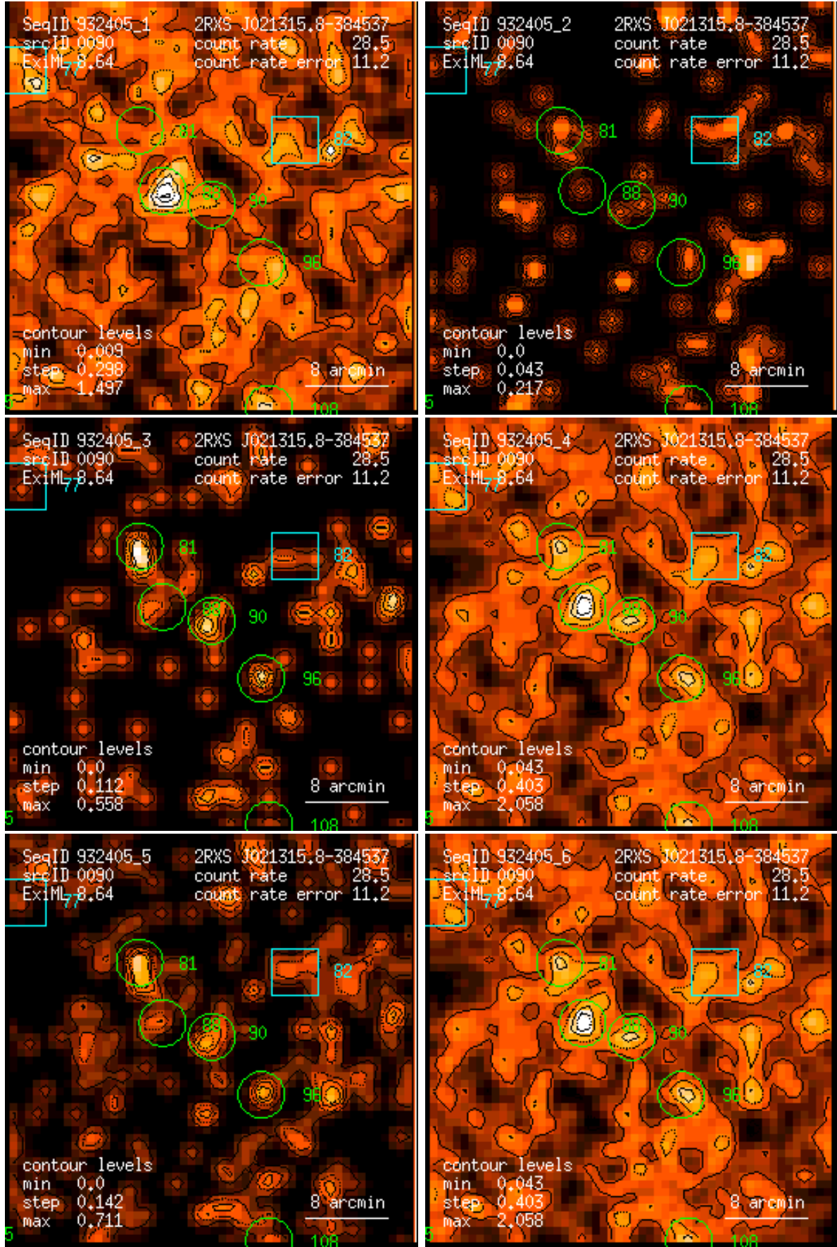
Figure 90: RASS 932405: detection 0090: band rate images, Gaussian filter: (1) PSPC channels 11 – 41, (2) 52 – 90, (3) 91 – 201, (4) 11 – 235, (5) 52 – 201, (6) 11 – 201. Broad band rates in counts/ks. Band rate contour levels in counts/ks/arcmin 2 .
