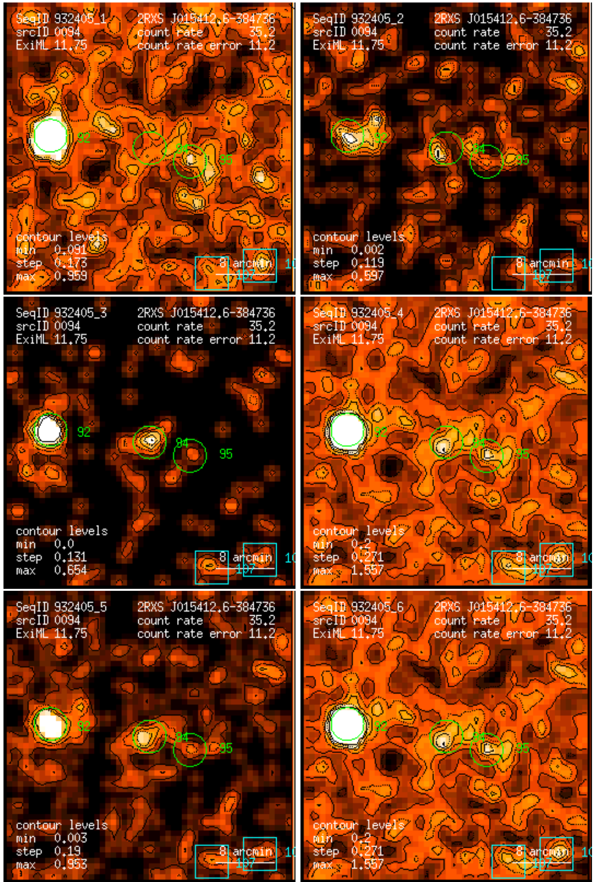
Figure 94: RASS 932405: detection 0094: band rate images, Gaussian filter: (1) PSPC channels 11 – 41, (2) 52 – 90, (3) 91 – 201, (4) 11 – 235, (5) 52 – 201, (6) 11 – 201. Broad band rates in counts/ks. Band rate contour levels in counts/ks/arcmin 2 .
